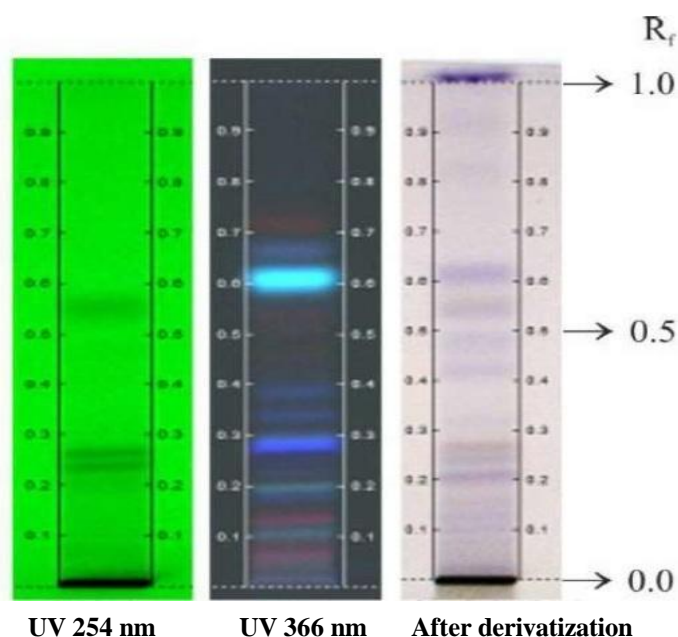
FIG. 3 TLC FINGERPRINTS OF SHEESHAM ( DALBERGIA SISSOO ROXB.) DRIED STEM BARK
