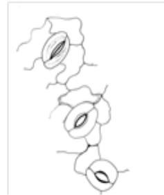
Anomocytic stomata
