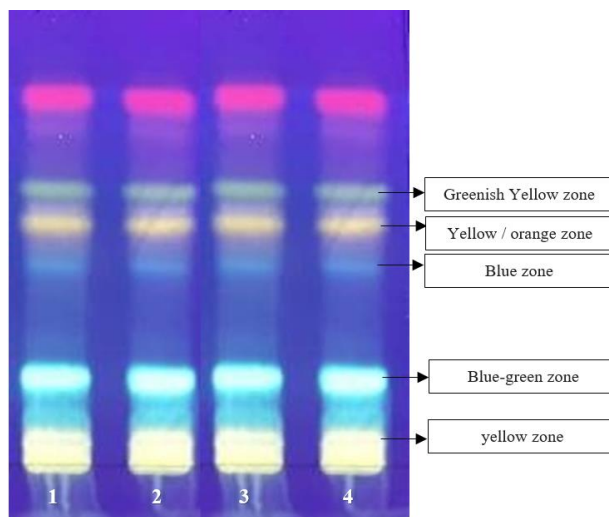
After derivatization with NP/PEG reagents TLC Profile of Achillea Millefolium Raw drug
