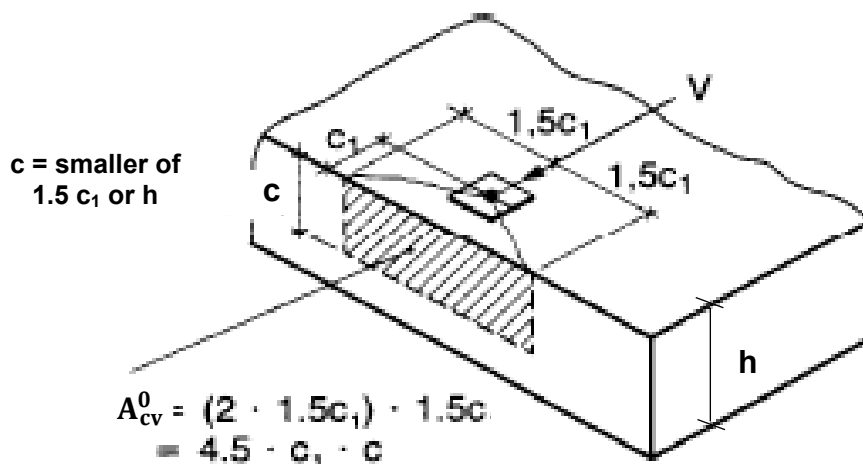
FIG. 37(A) IDEALISED CONCRETE CONE FOR EDGE SHEAR
