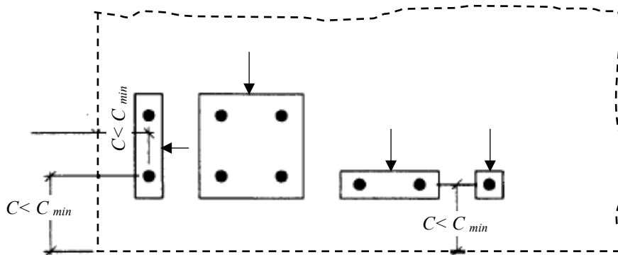
Fig. 34 (b) Anchorages Situated Near to Concrete Edges
