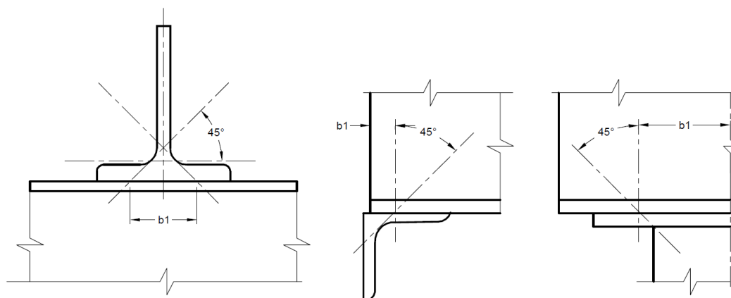
FIG. 15 STIFF BEARING LENGTH, b_1
