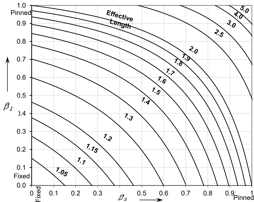
FIG. 28 COLUMN EFFECTIVE LENGTH FACTOR - SWAY FRAME (Clause B-2.1)
