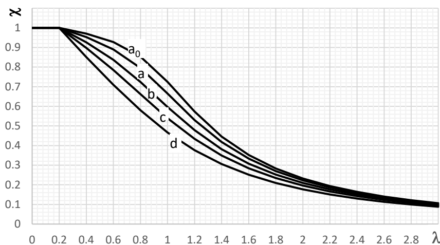
FIG. 8 BUCKLING CURVES
