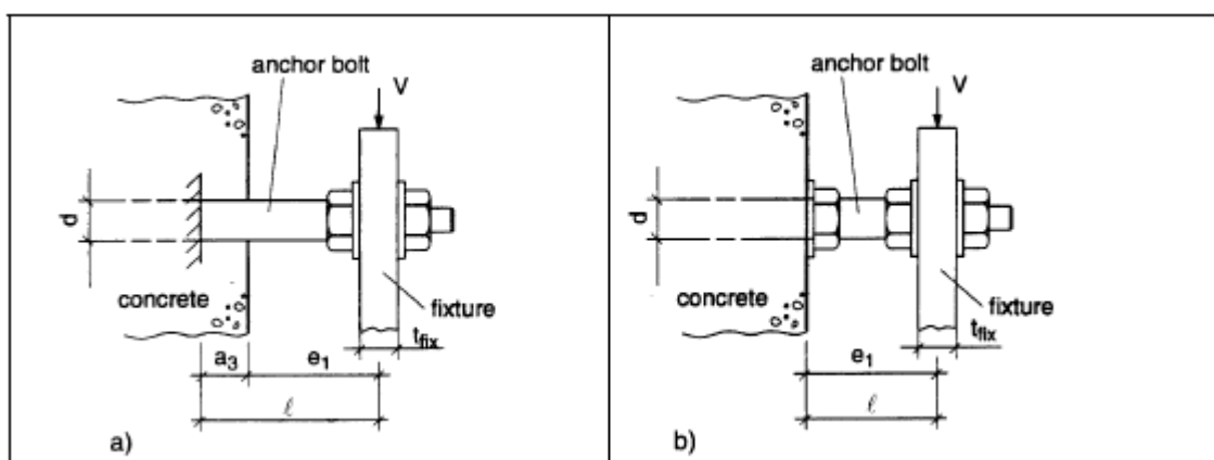
FIG. 36 LEVER ARM, l , OF ANCHOR
