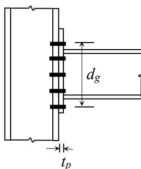
32E End plate without column stiffeners
