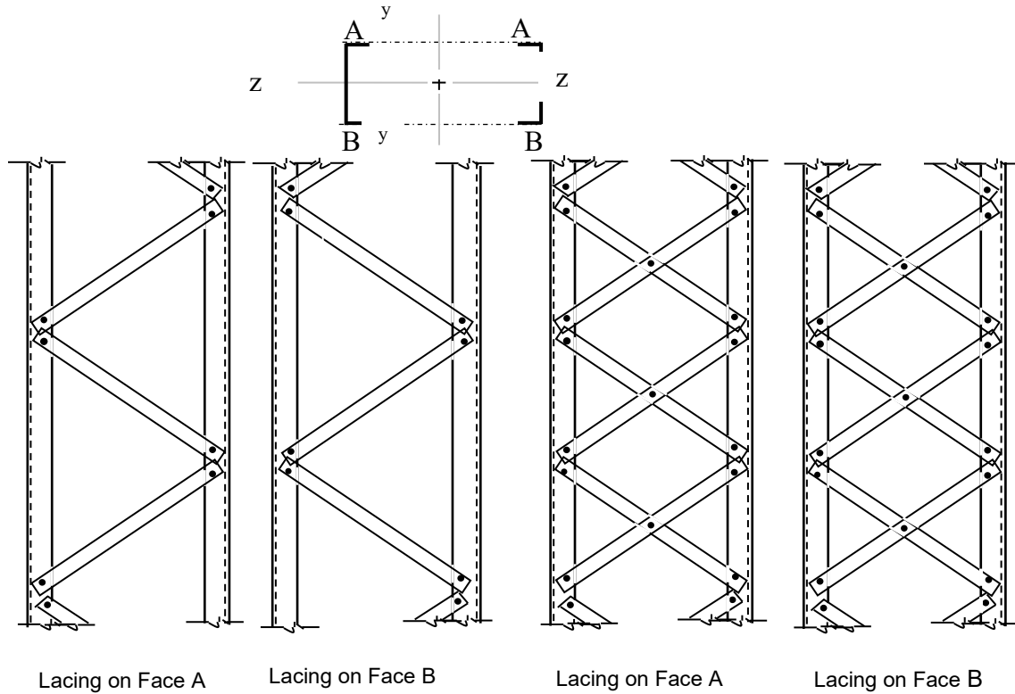
Preferred Lacing Arrangement
