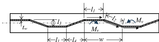
FIG. 39 IN-PLANE TRANSVERSE BENDING MOMENT IN FLANGES DUE ECCENTRIC SHEAR FLOW FROM THE WEB
