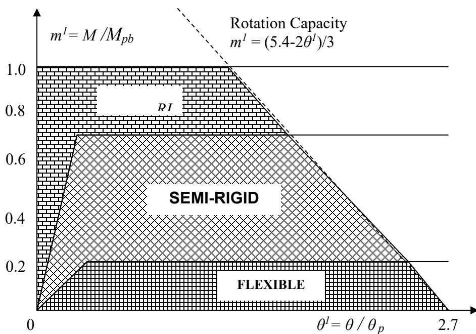
FIG. 33 CLASSIFICATION OF CONNECTIONS ACCORDING TO BJORHOVDE
