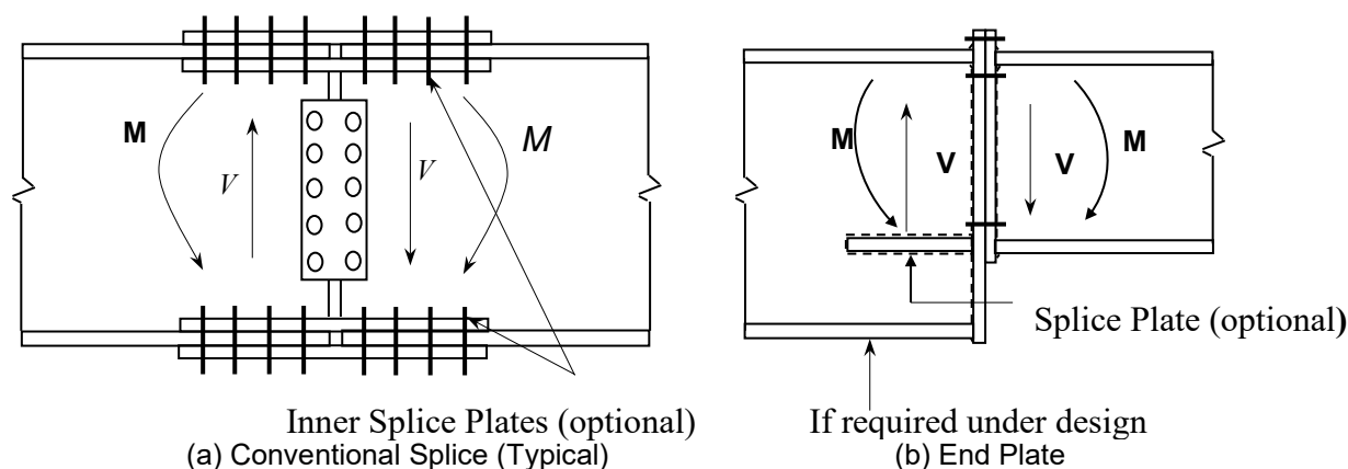
FIG. 30 BEAM SPLICES
