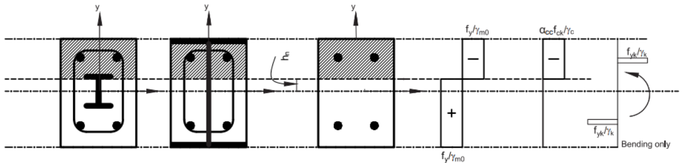
FIG. 42 STRESS DISTRIBUTION AT ULTIMATE STAGE UNDER ONLY BENDING MOMENT
