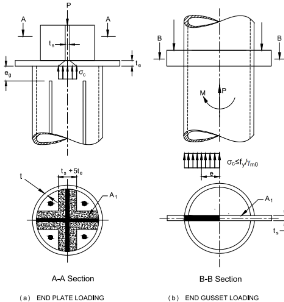
FIG. 20 PARTIALLY LOADED CIRCULAR CONCRETE FILLED HOLLOW SECTION
