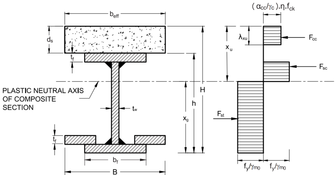
FIG 30 STRESS DIAGRAM FOR FILLER BEAM
