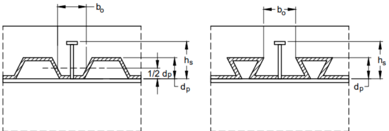
FIG.10 BEAM WITH PROFILED DECKING SHEET RIBS TRANSVERSE TO THE BEAM
