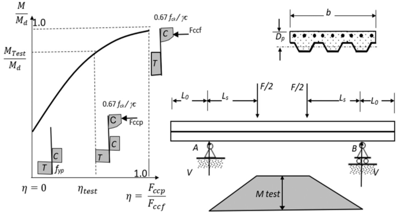
FIG. 39 TEST TO DETERMINATION OF THE DEGREE OF THE PARTIAL SHEAR CONNECTION
