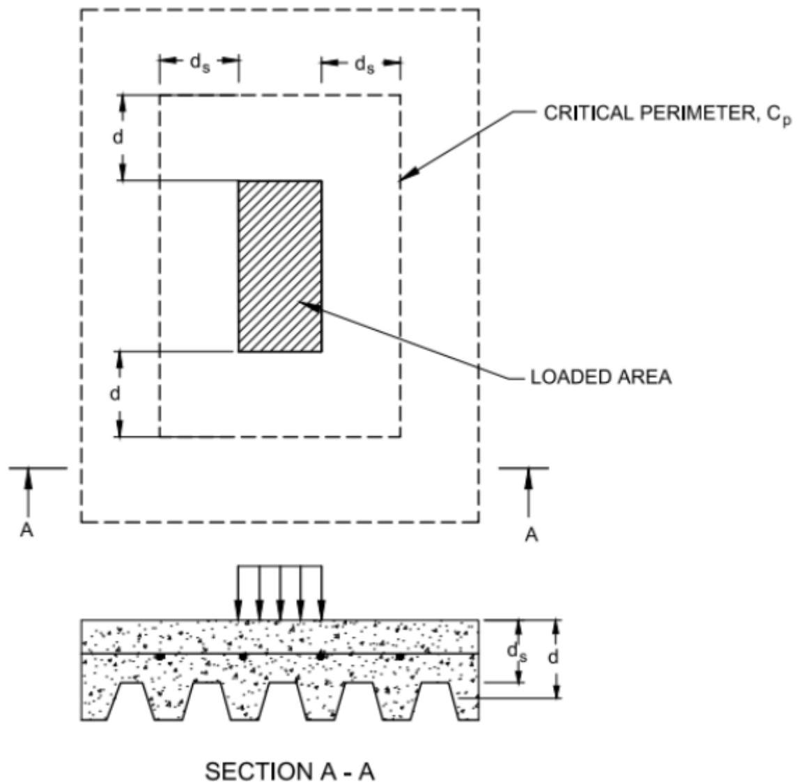
FIG. 17 PUNCHING PERIMETER IN A PROFILED COMPOSITE SLAB
