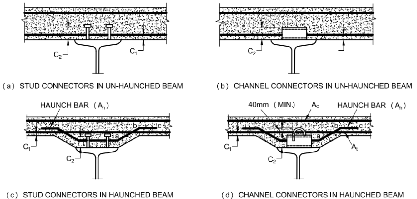
FIG. 13 ARRANGEMENT OF TRANSVERSE REINFORCEMENTS
