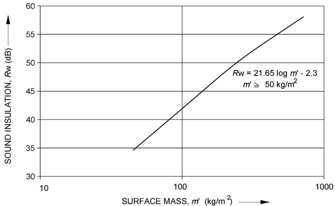
FIG. 8 MASS LAW CURVE
