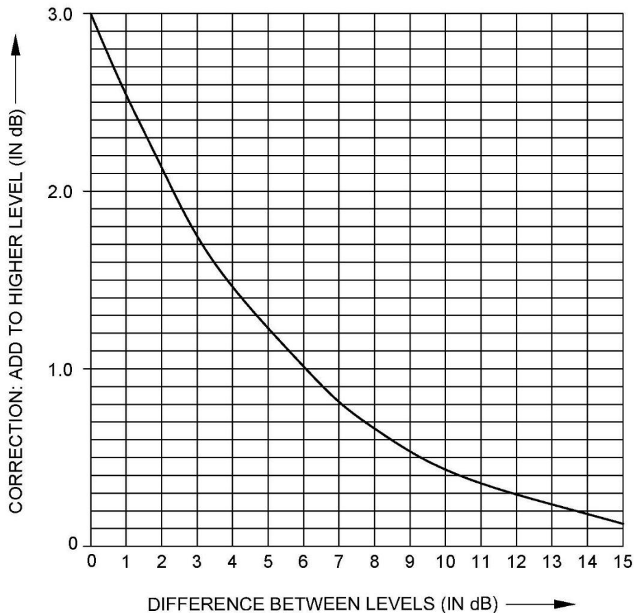
FIG. 3 ADDITION OF TWO NOISE LEVELS
