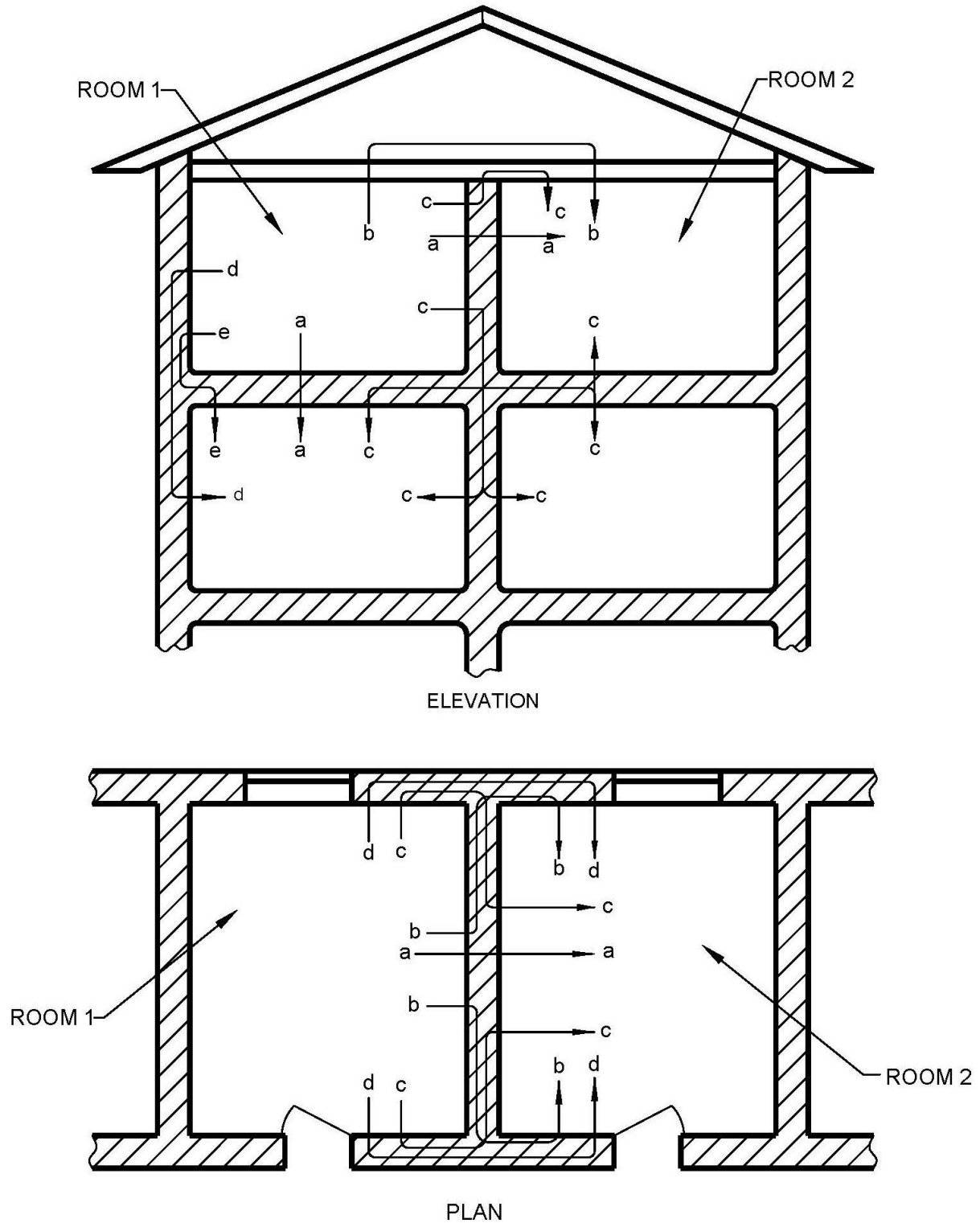
FIG. 6 TRANSMISSION PATHS (VIA THE STRUCTURE) OF NOISE ORIGINATING IN ROOM 1 (DIAGRAMMATIC)
