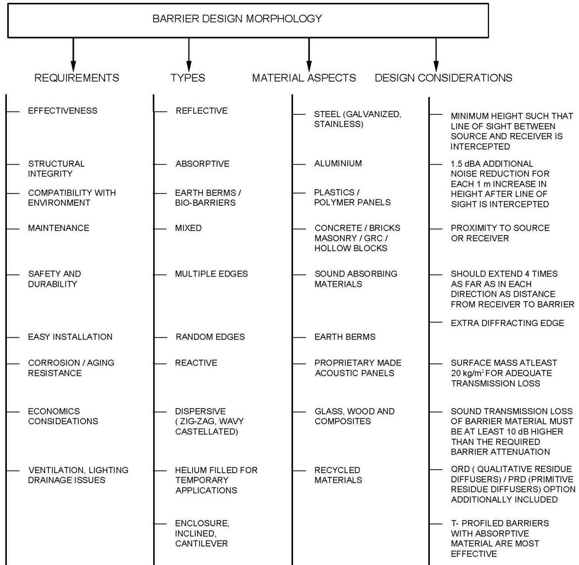
FIG. 9 DESIGN MORPHOLOGY FOR NOISE BARRIERS
