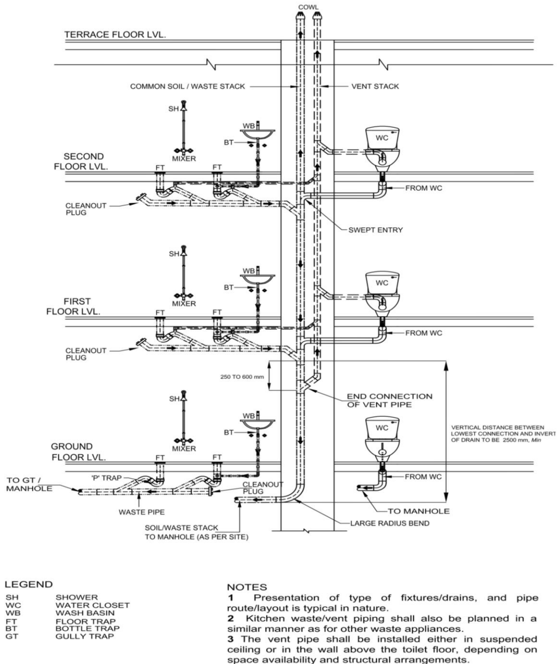
FIG. 3 ONE PIPE – FULLY VENTILATED SYSTEM
