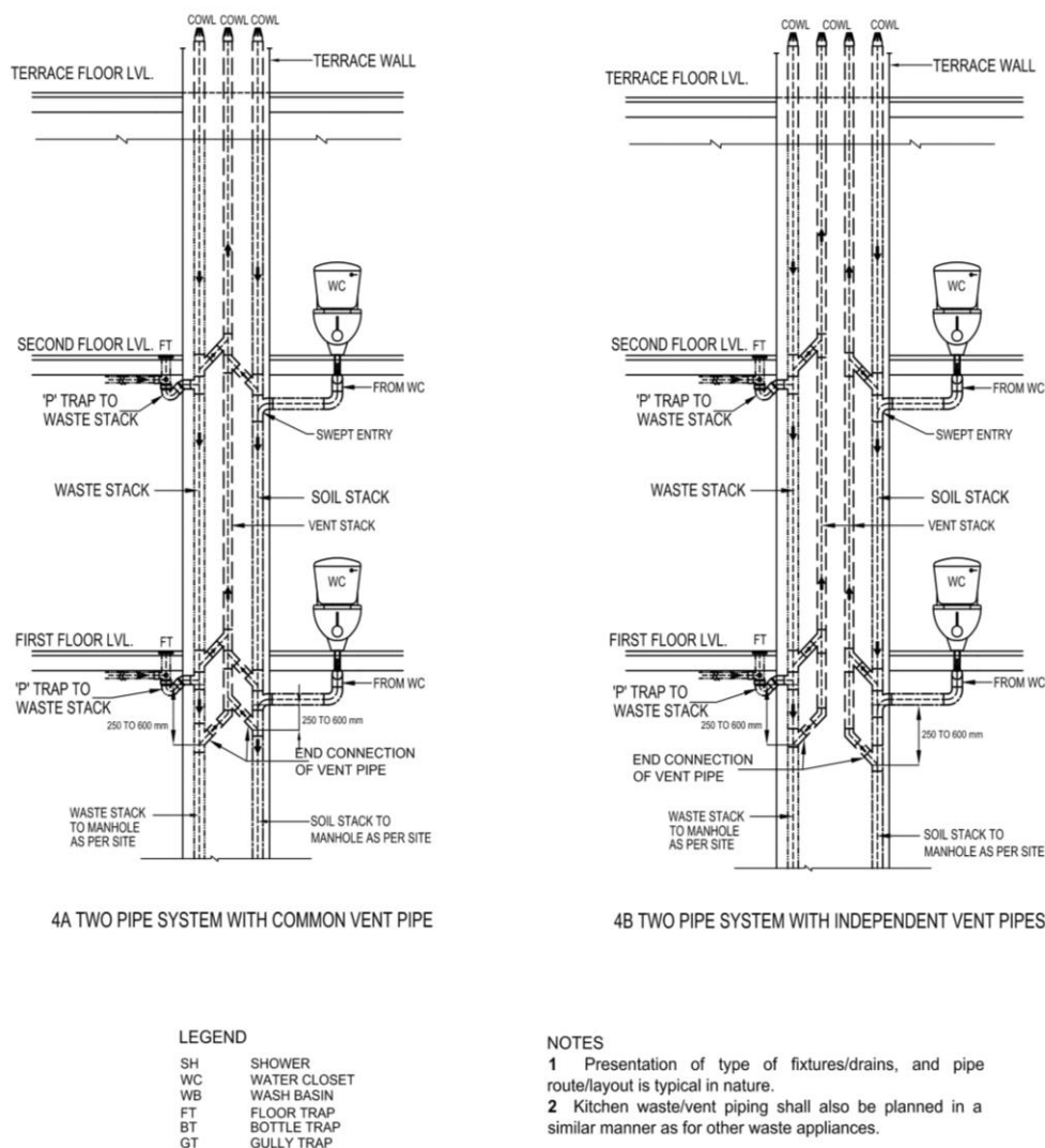
FIG. 4 TWO PIPE SYSTEM
