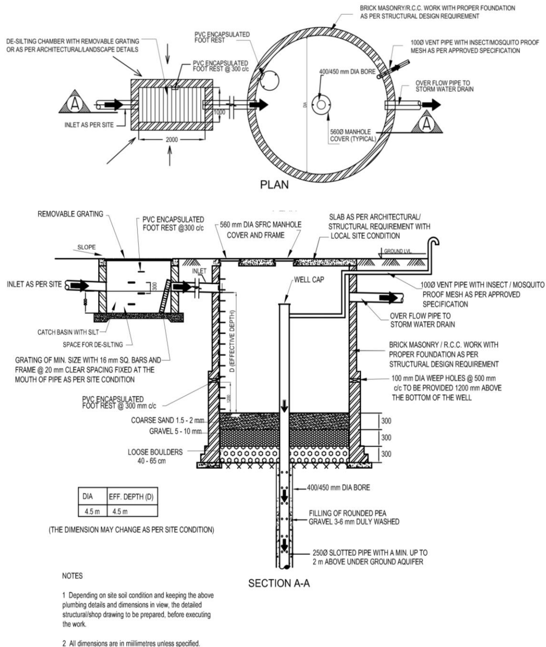
FIG. 12 ARTIFICIAL GROUND WATER RECHARGE STRUCTURE
