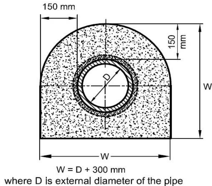
FIG. 17 SURROUND OR ENCASING
