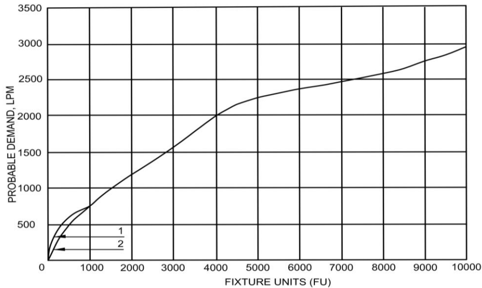
6A GRAPH FOR PROBABLE DEMAND UP TO 10 000 FU
