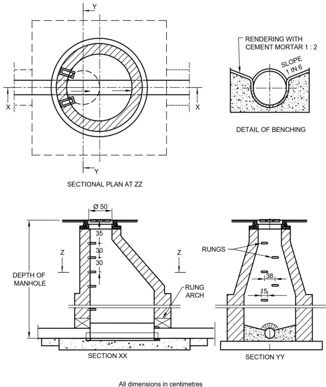
FIG. 9 DETAIL OF MANHOLE (DEPTH 2.5 m AND ABOVE)
