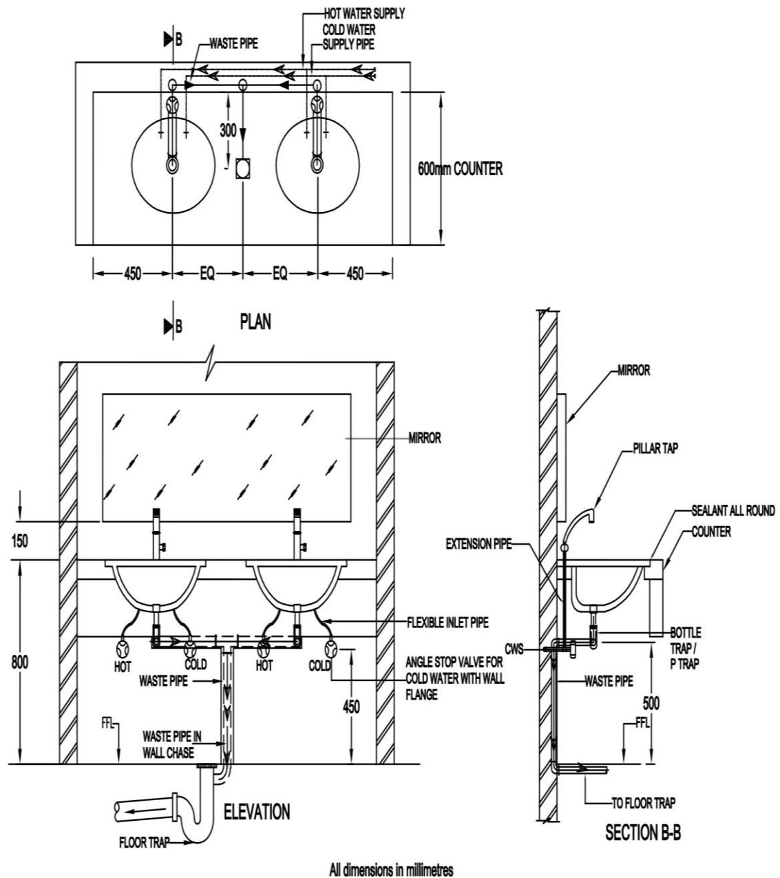
FIG. 21 OVAL WASH BASIN (BELOW COUNTER)
