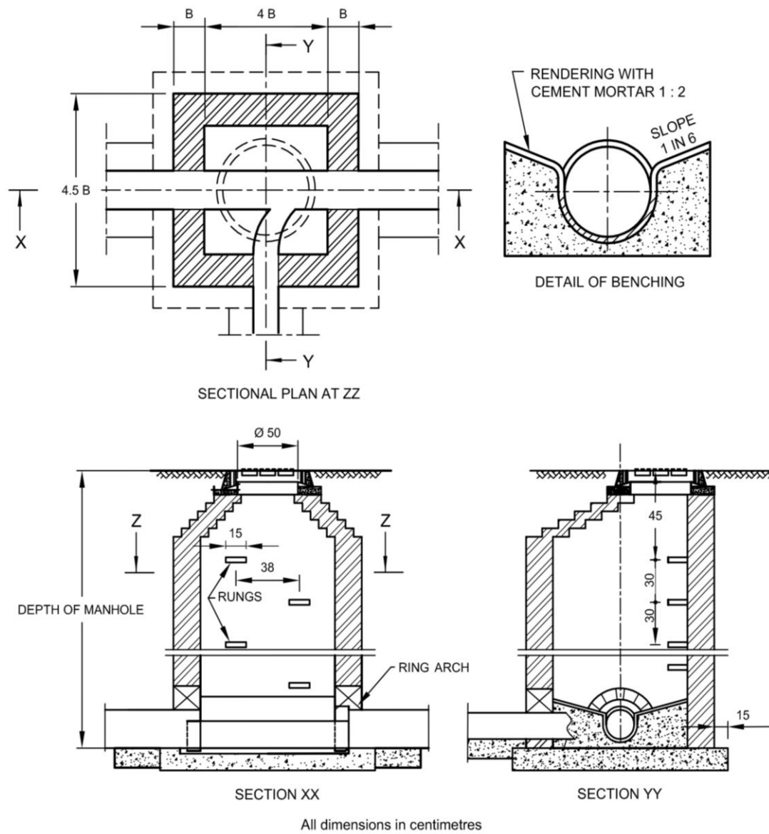
FIG. 8 DETAIL OF MANHOLE (DEPTH FROM 0.9 m AND UP TO 2.5 m)
