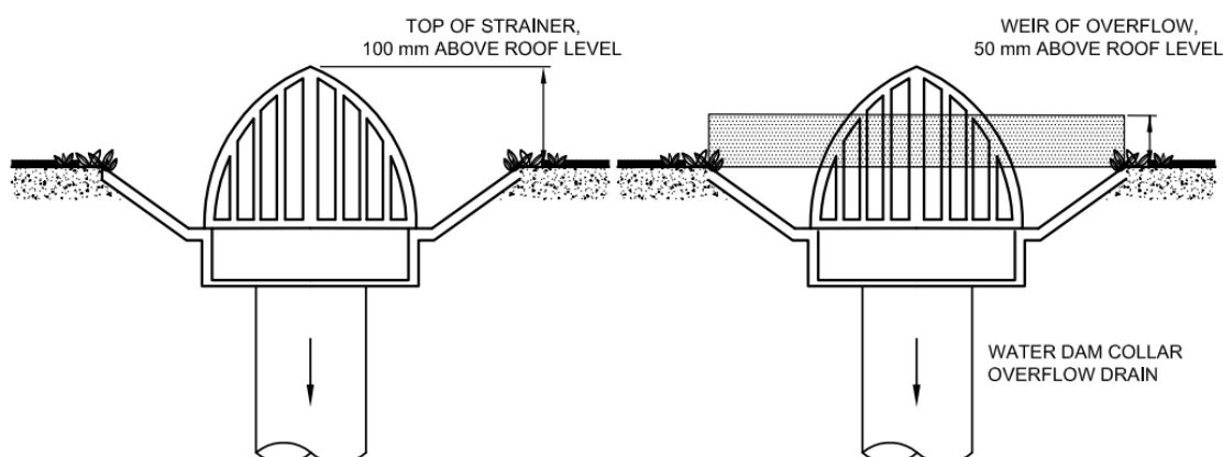
11A TYPICAL VIEW OF ROOF DRAIN (LEFT) AND ROOF DRAIN WITH WEIR (RIGHT)
