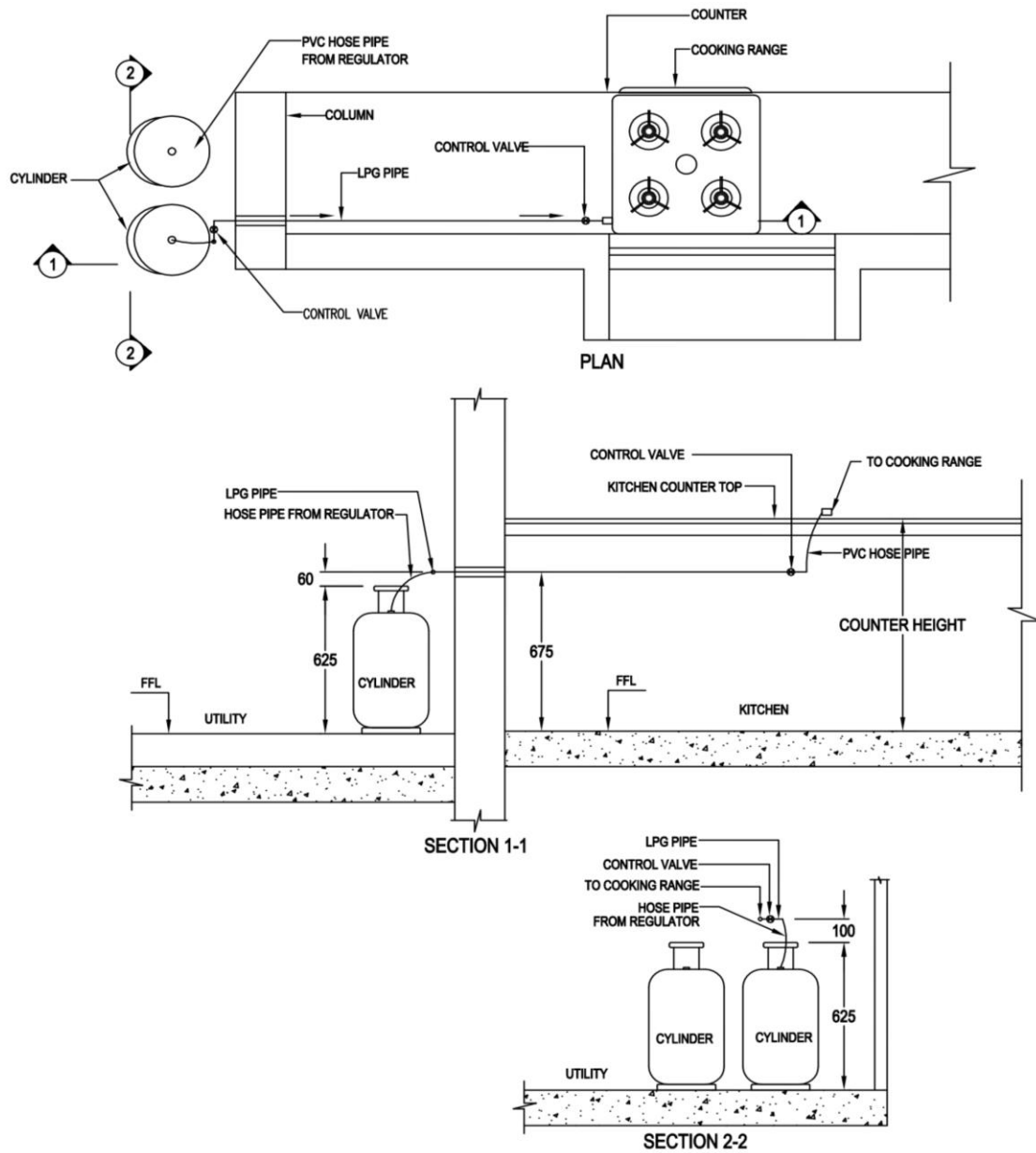
FIG. 32 LPG PIPING
