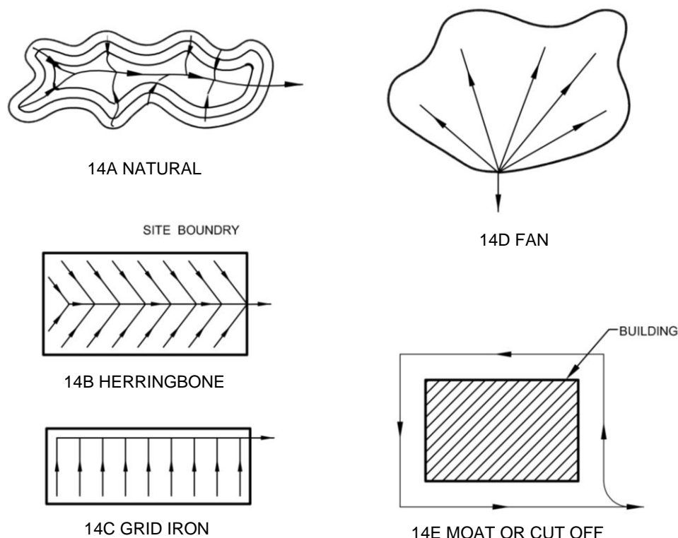
FIG. 14 DETAILS OF SUBSOIL DRAINAGE SYSTEM
