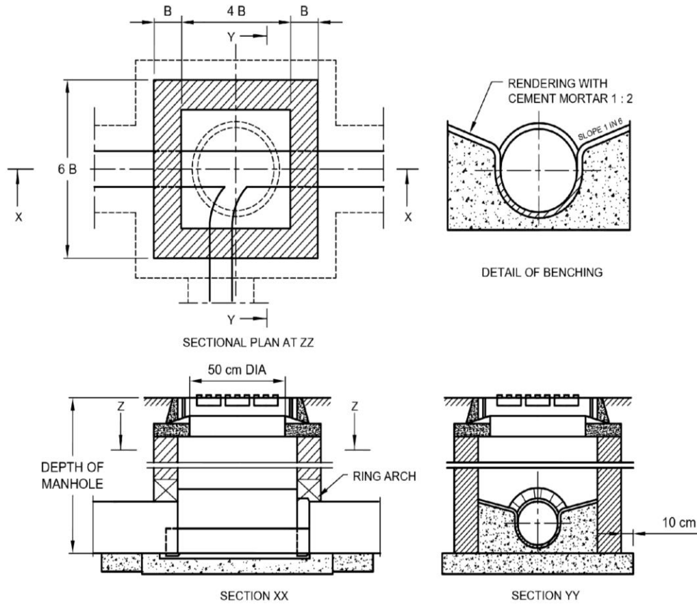
FIG. 7 DETAIL OF MANHOLE (DEPTH LESS THAN 0.90 m)
