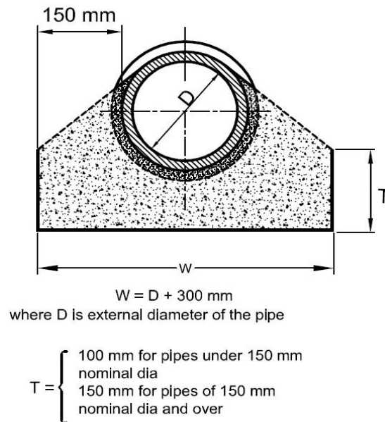
FIG. 16 HAUNCHING
