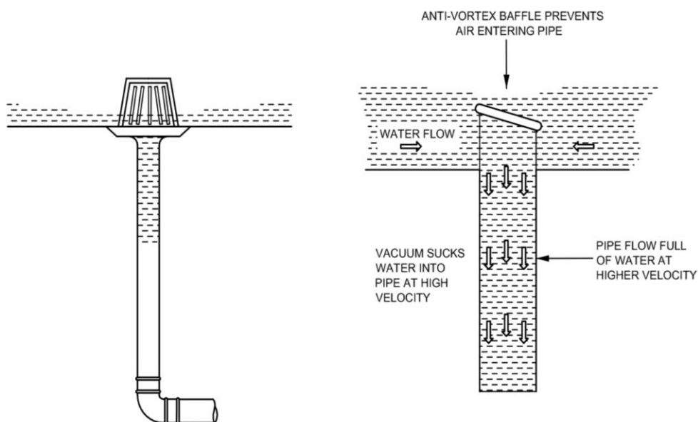
FIG. 13 SIPHONIC DRAINAGE SYSTEM
