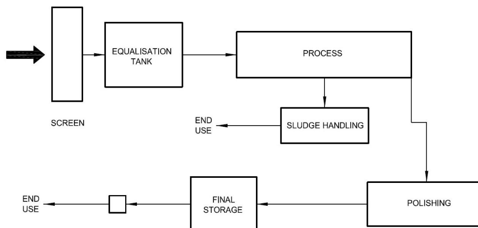
FIG. 18 TYPICAL SCHEME FOR SEWAGE TREATMENT
