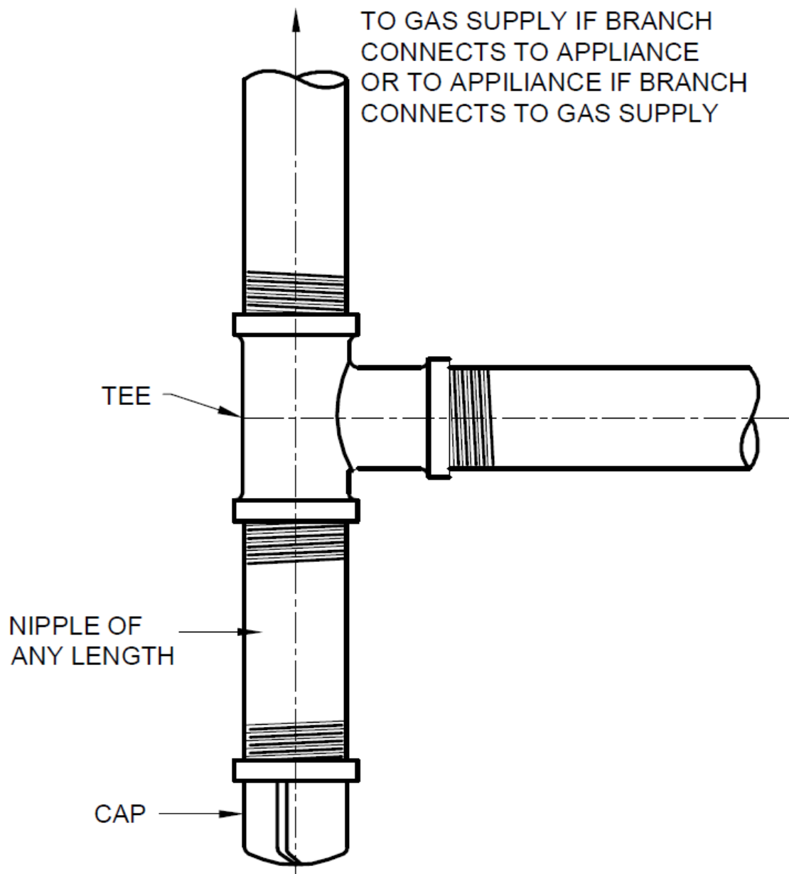
FIG. 1 METHOD OF INSTALLING A TEE FITTING SEDIMENT TRAP
