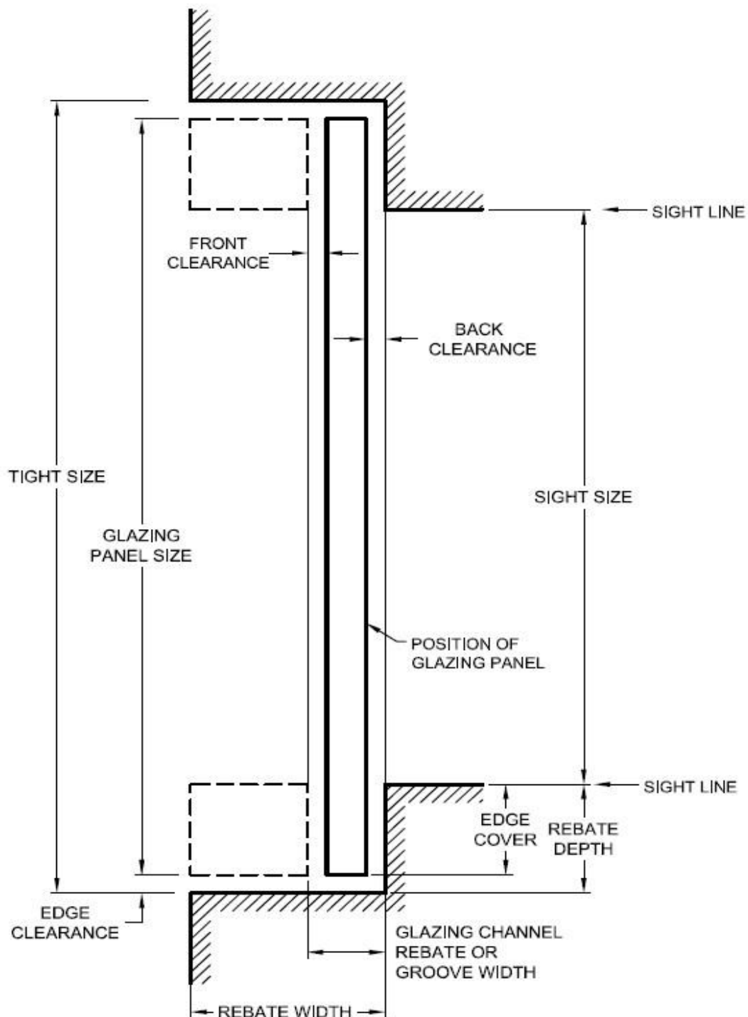
FIG. 2 SIZES AND REBATES
