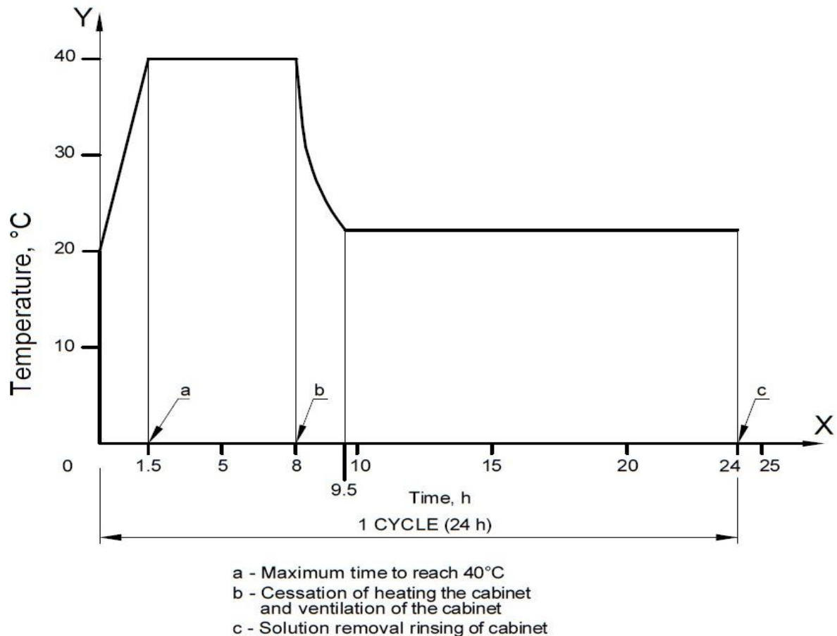
FIG. 19 24-HOUR CYCLE OF HEATING
