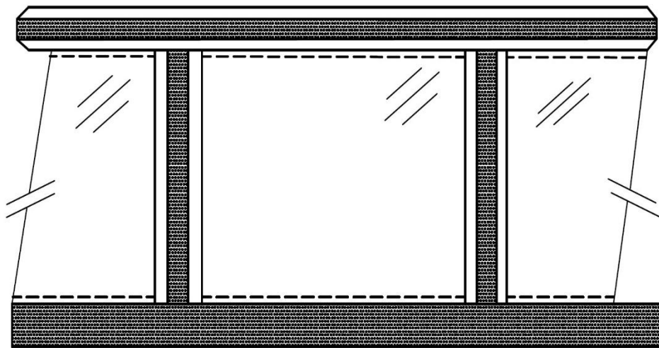
FIG. 25 GLASS SUPPORTED ON HORIZONTAL EDGES ONLY
