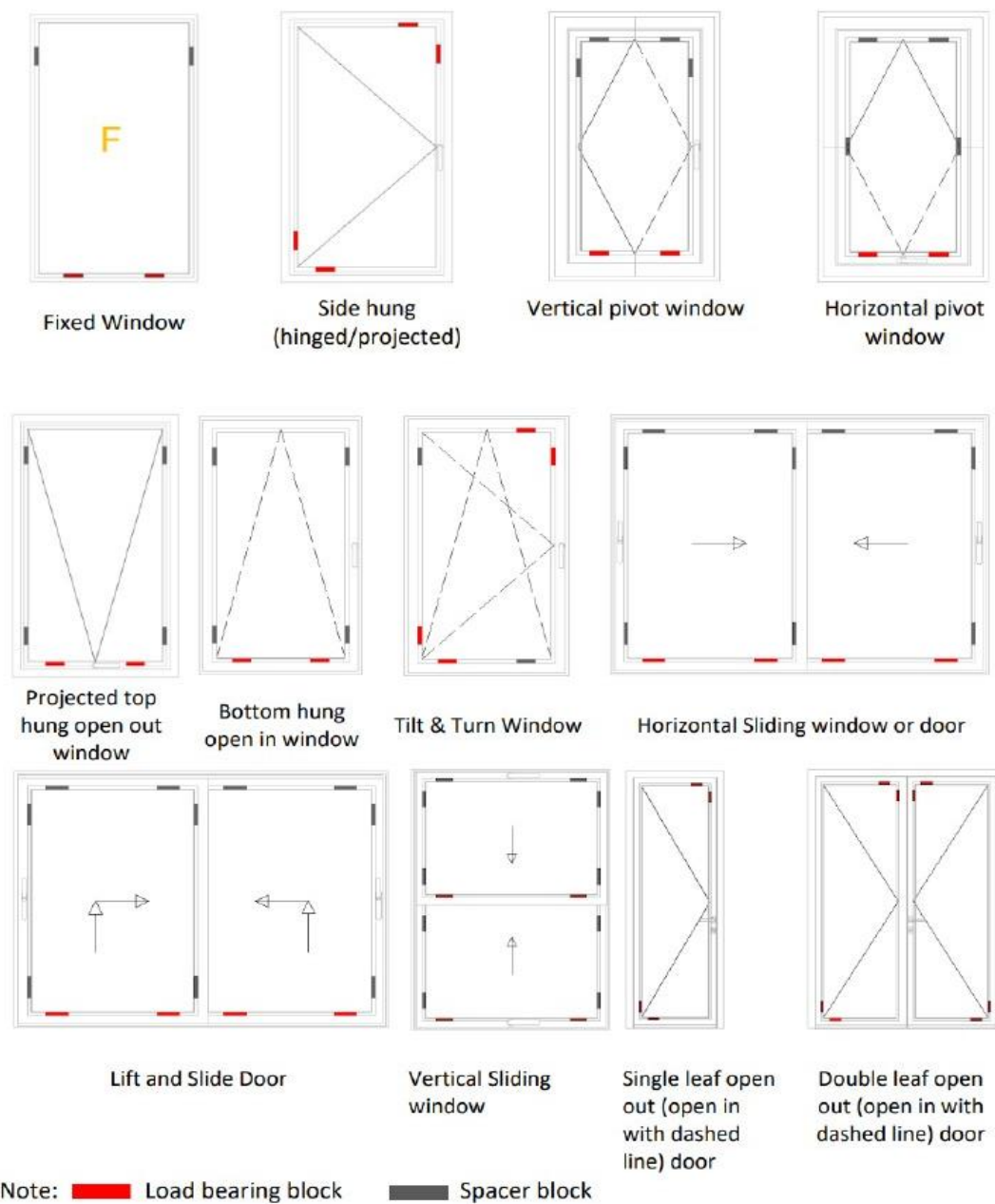
FIG. 15 NUMBER AND POSITION OF SETTING AND LOCATION/GLAZING BLOCK
