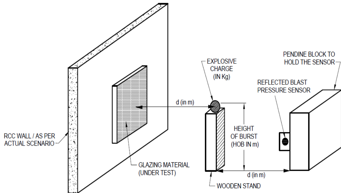
FIG. 34 ISOMETRIC VIEW – SCHEMATIC OF TEST SETUP
