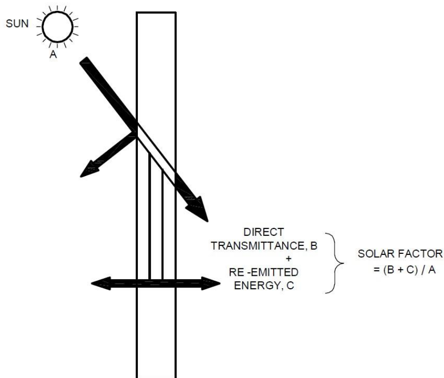
FIG. 6 SOLAR HEAT GAIN COEFFICIENT
