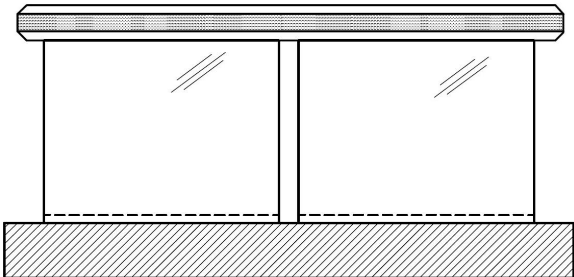
FIG. 28 FREE STANDING GLASS PROTECTIVE RAILING
