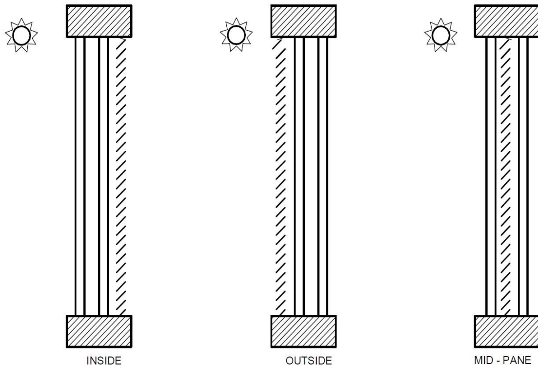
FIG. 11 PLACEMENT OF SHADING DEVICES FOR OPTIMAL SUN CONTROL IN GLAZING SYSTEMS
