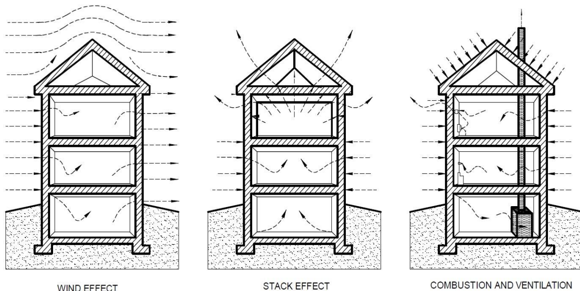
FIG. 12 MECHANISMS OF AIR INFILTRATION: WIND EFFECT, STACK EFFECT, AND COMBUSTION AND VENTILATION IN BUILDING ENCLOSURES
