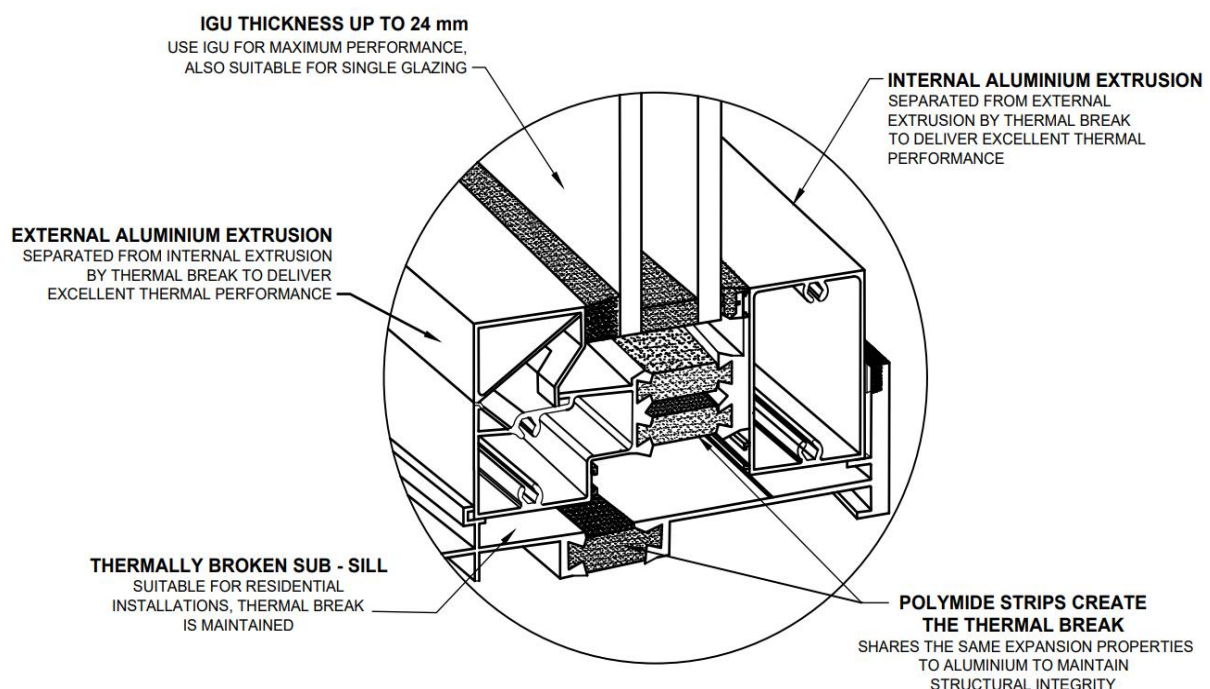
FIG. 10 THERMALLY BROKEN ALUMINIUM FRAME ASSEMBLY FOR IMPROVED THERMAL PERFORMANCE IN GLAZING SYSTEMS
