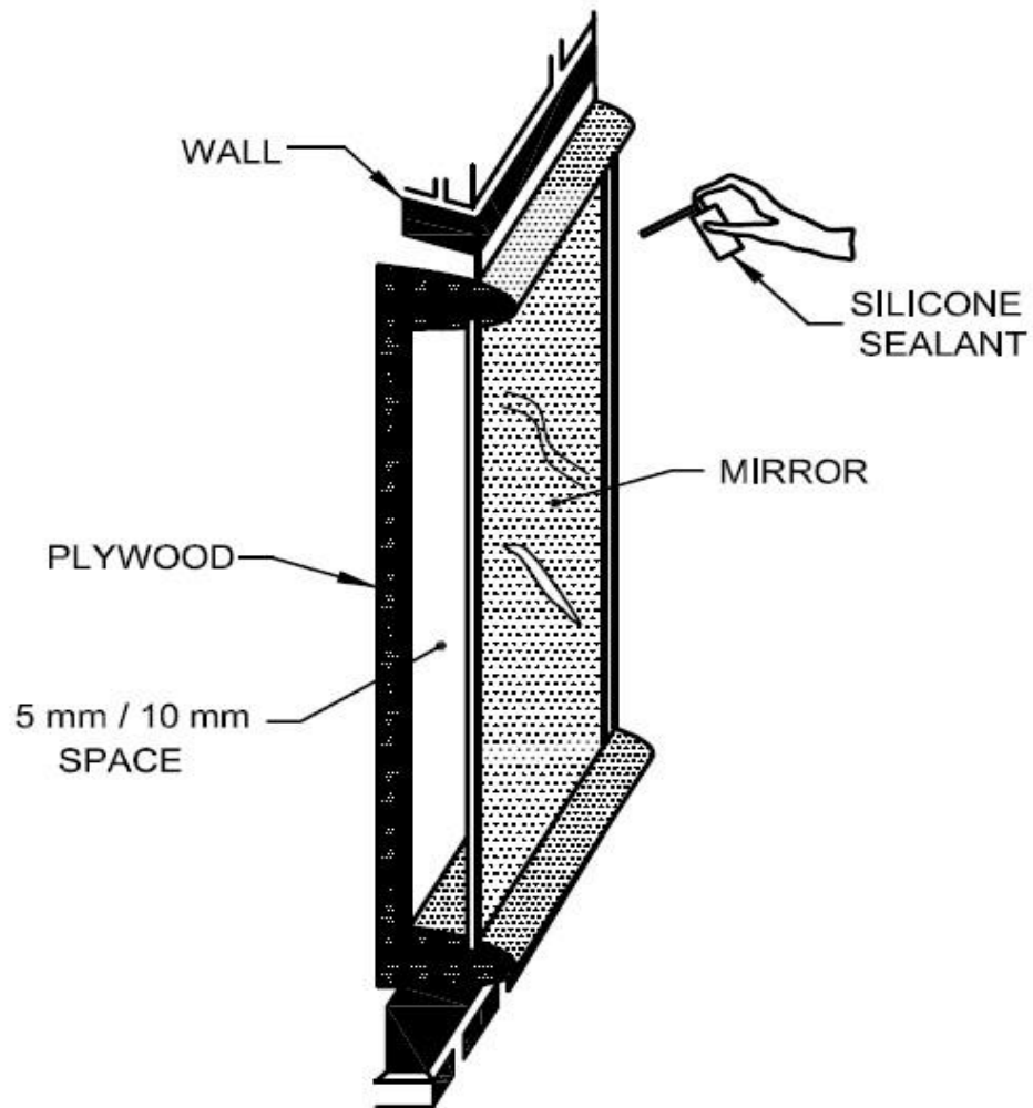
FIG. 20 INSTALLATION OF MIRRORS
