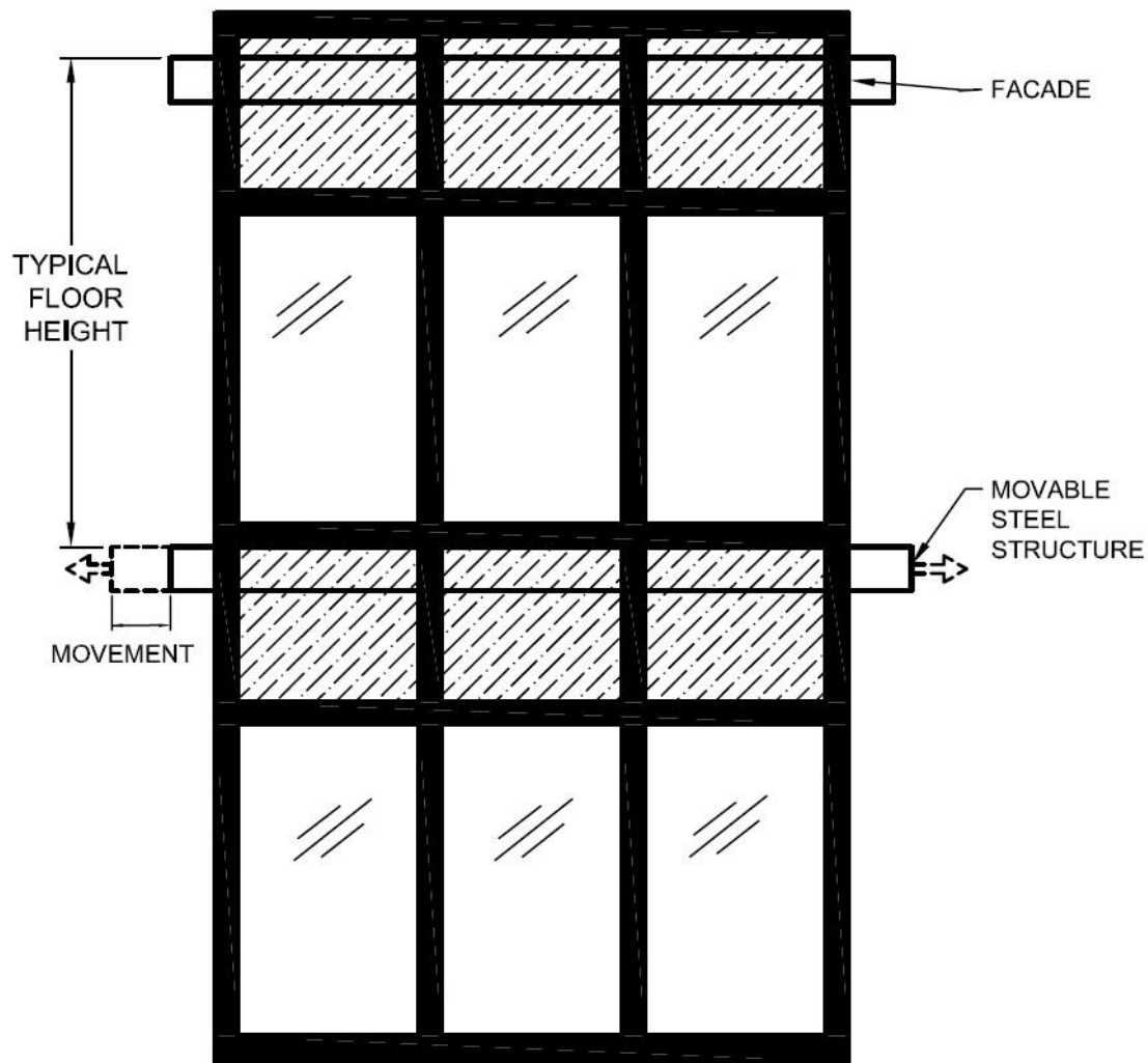
FIG. 33 ILLUSTRATION OF MOVABLE STRUCTURAL ELEMENTS IN CURTAIN WALL SYSTEMS UNDER INTER-STOREY DRIFT CONDITIONS
