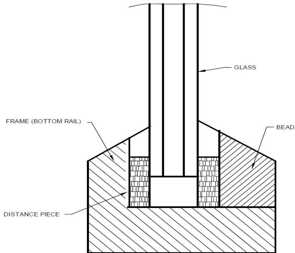
FIG. 16 POSITION OF DISTANCE PIECES
