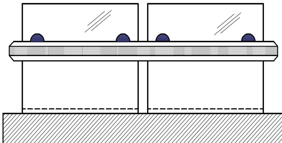
FIG. 30 BOTTOM SUPPORTED WITH SURFACE ATTACHED / BOLTED HANDRAIL – GLAZING AS STRUCTURAL MEMBER.
