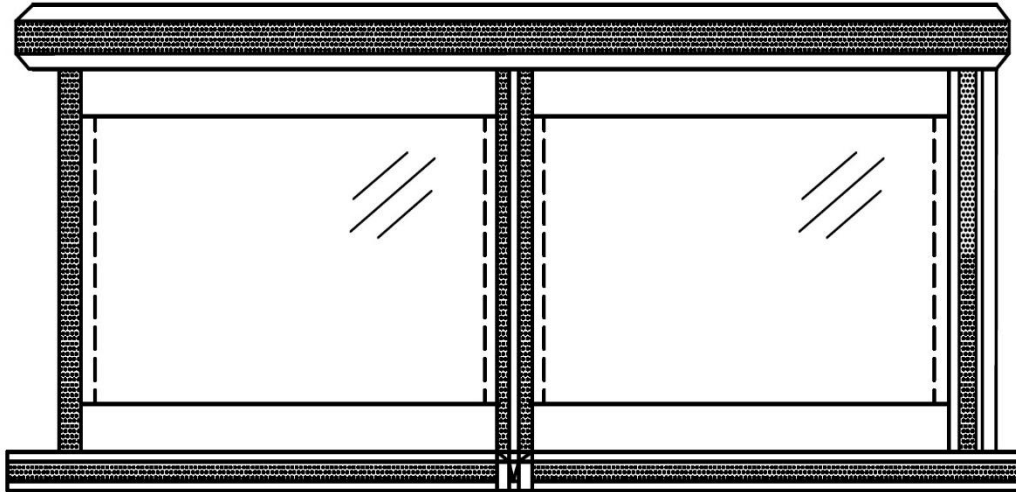
FIG. 26 GLASS SUPPORTED ON ALL FOUR EDGES
