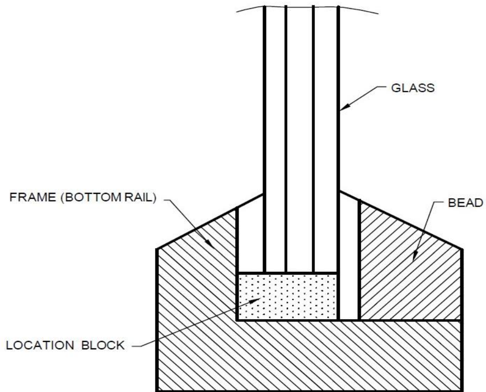
FIG. 14 POSITION OF LOCATION BLOCK
