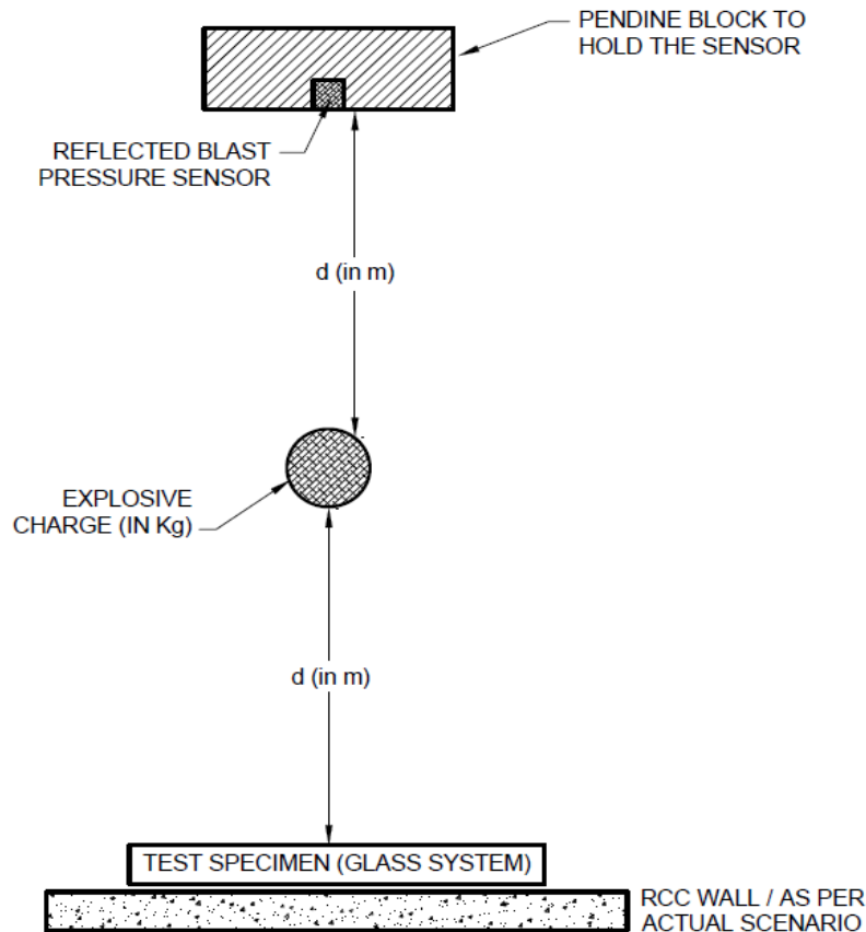
FIG. 35 TOP VIEW – SCHEMATIC OF TEST SETUP
