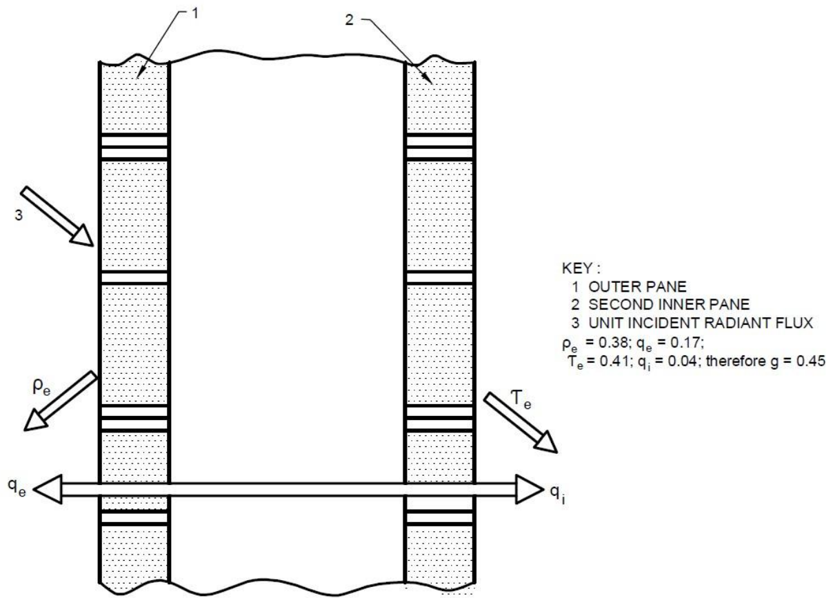
FIG. 7 COMPONENTS OF INCIDENT SOLAR RADIANT FLUX
