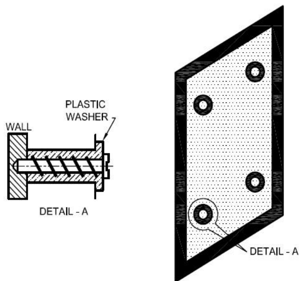
FIG. 21 DETAILS OF USE OF SCREWS AND INTERLEAVING WASHERS FOR INSTALLING MIRRORS
