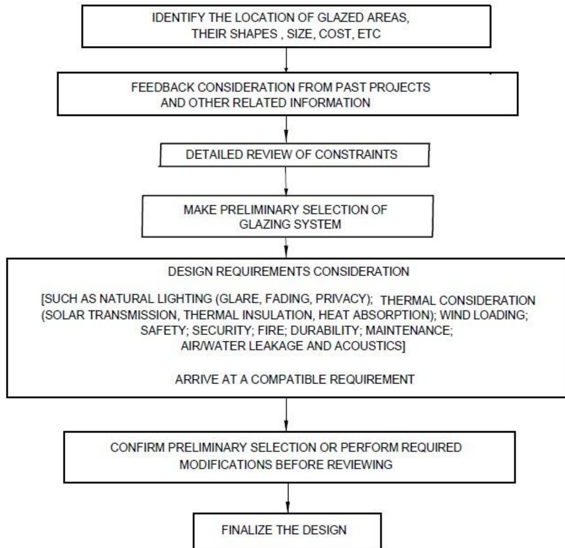
FIG. 1 TYPICAL SEQUENCE OF DESIGN EVALUATION FOR GLAZED AREAS
