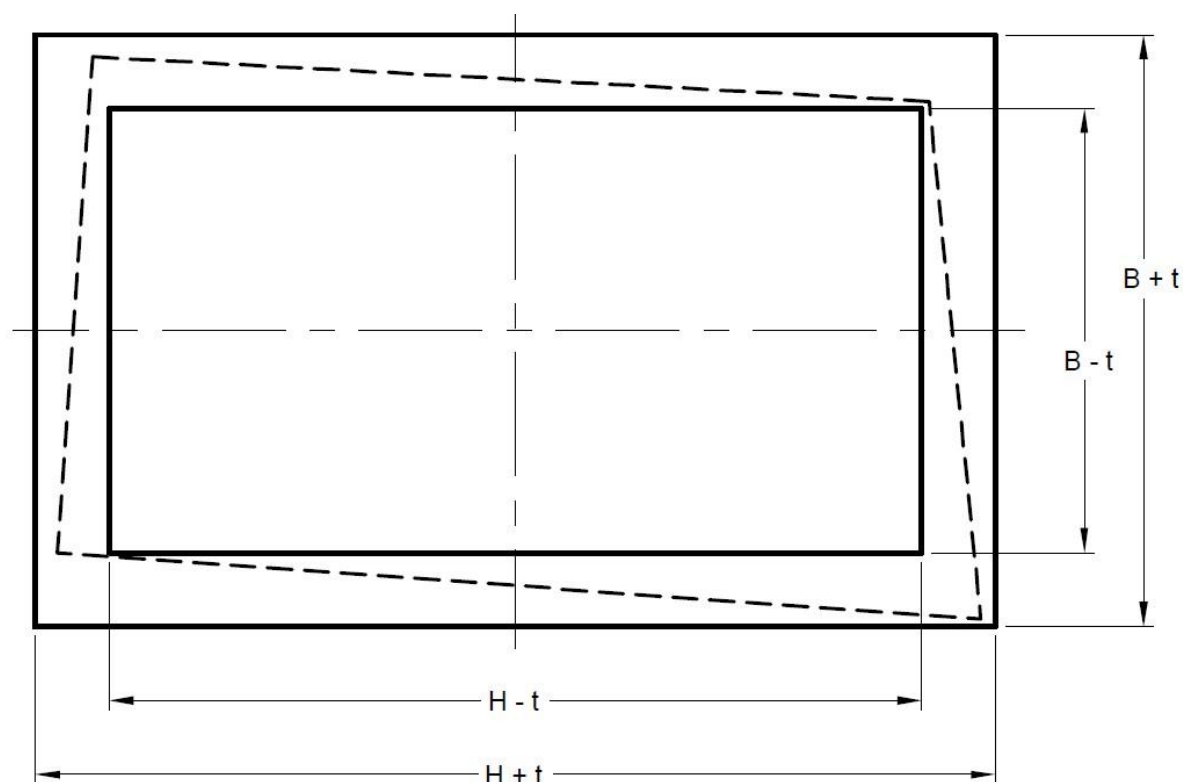
FIG. 5 TOLERANCE ( t ) FOR WIDTH ( B ) AND LENGTH ( H )
