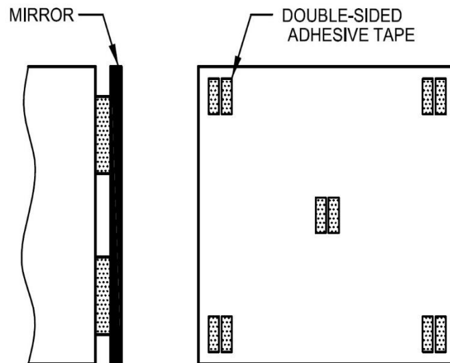
FIG. 22 DETAILS OF USE OF DOUBLE SIDED ADHESIVE TAPES FOR INSTALLING MIRRORS
