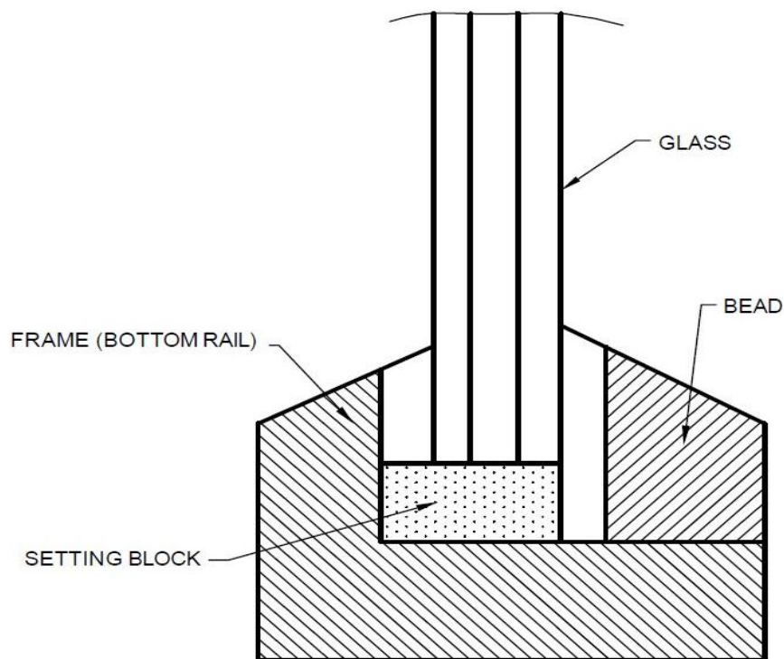
FIG. 13 POSITION OF SETTING BLOCK
