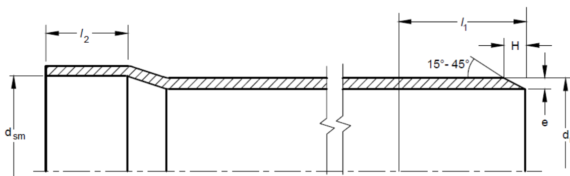
FIG. 5 BASIC DIMENSIONS FOR INTEGRAL SOCKETS AND SPIGOTS FOR SOLVENT-CEMENTED JOINTS
