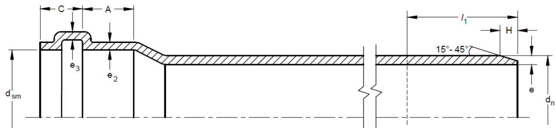
FIG. 2 BASIC DIMENSIONS OF INTERNAL SOCKETS AND SPIGOT ENDS FOR ELASTOMETRIC SEALING RING JOINTS
