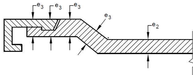
FIG. 3 EXAMPLE OF A SEAL RETAINING CAP AND CALCULATION OF THE WALL THICKNESS OF SOCKETS
