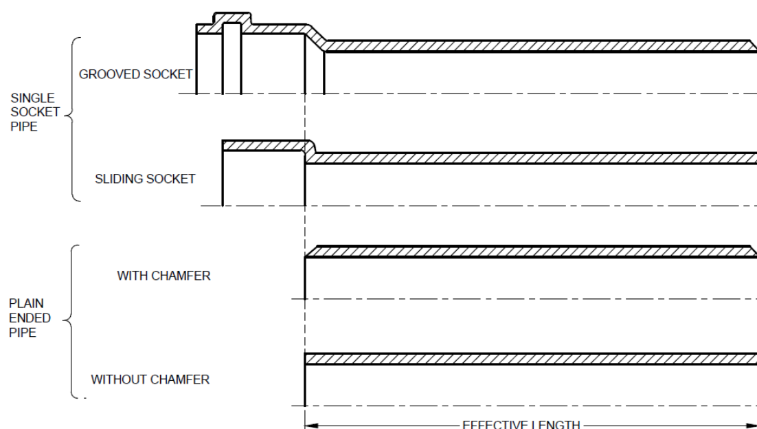
FIG. 1 EFFECTIVE LENGTH OF PIPES
