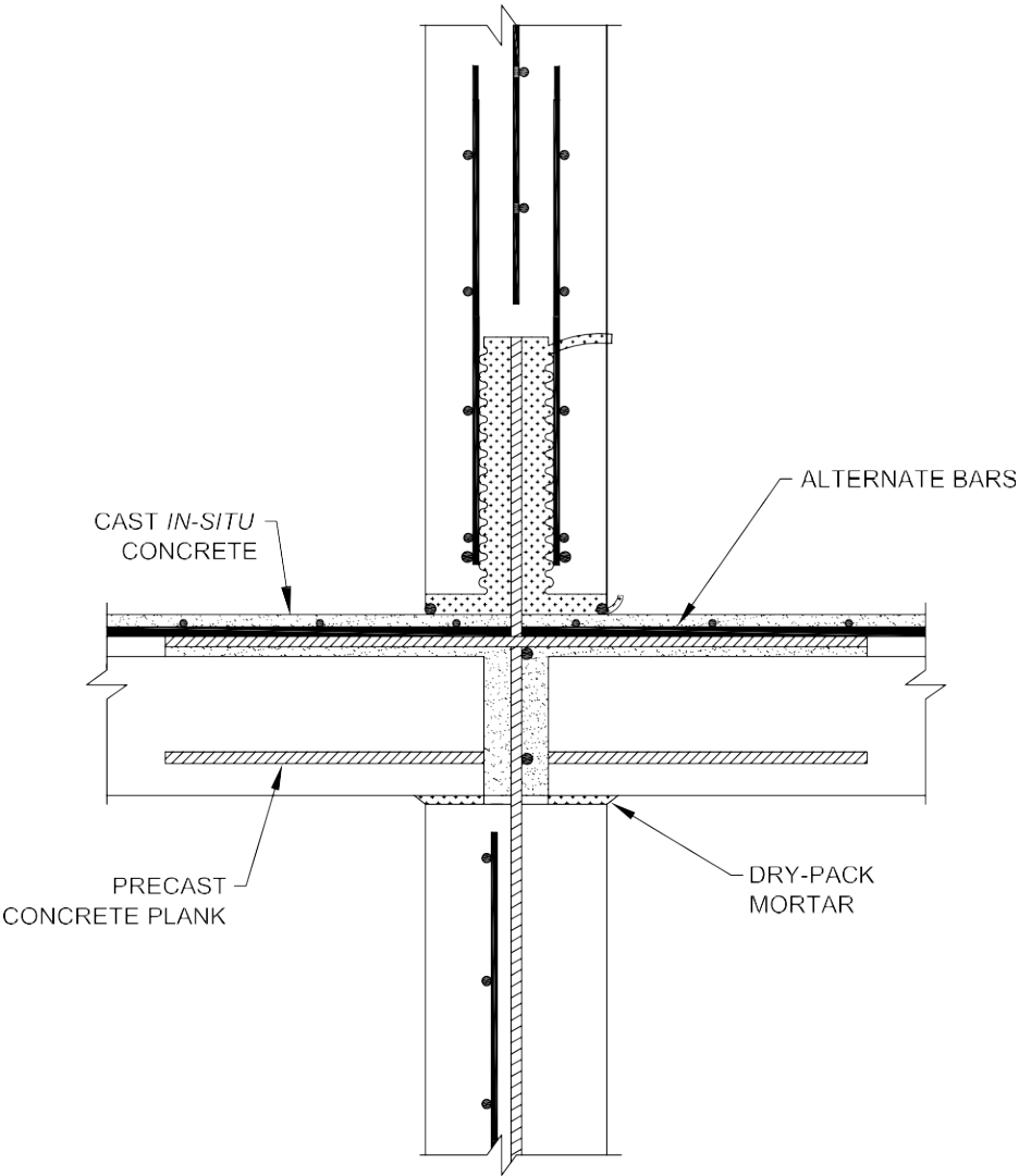
FIG. 53 WALL TO FLOOR SLAB CONNECTION
