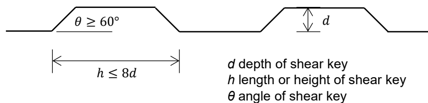
FIG. 31 DETAILING OF SHEAR KEY WITHOUT REINFORCEMENT
