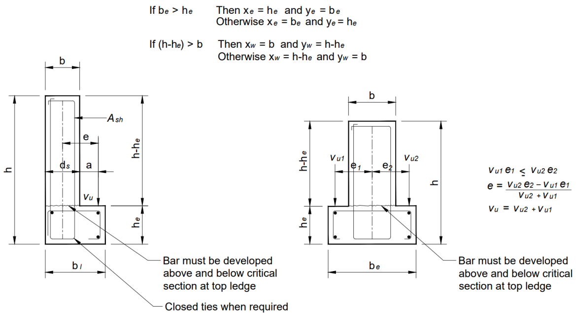
FIG. 27 LEDGE HANGER STEEL GEOMETRY
