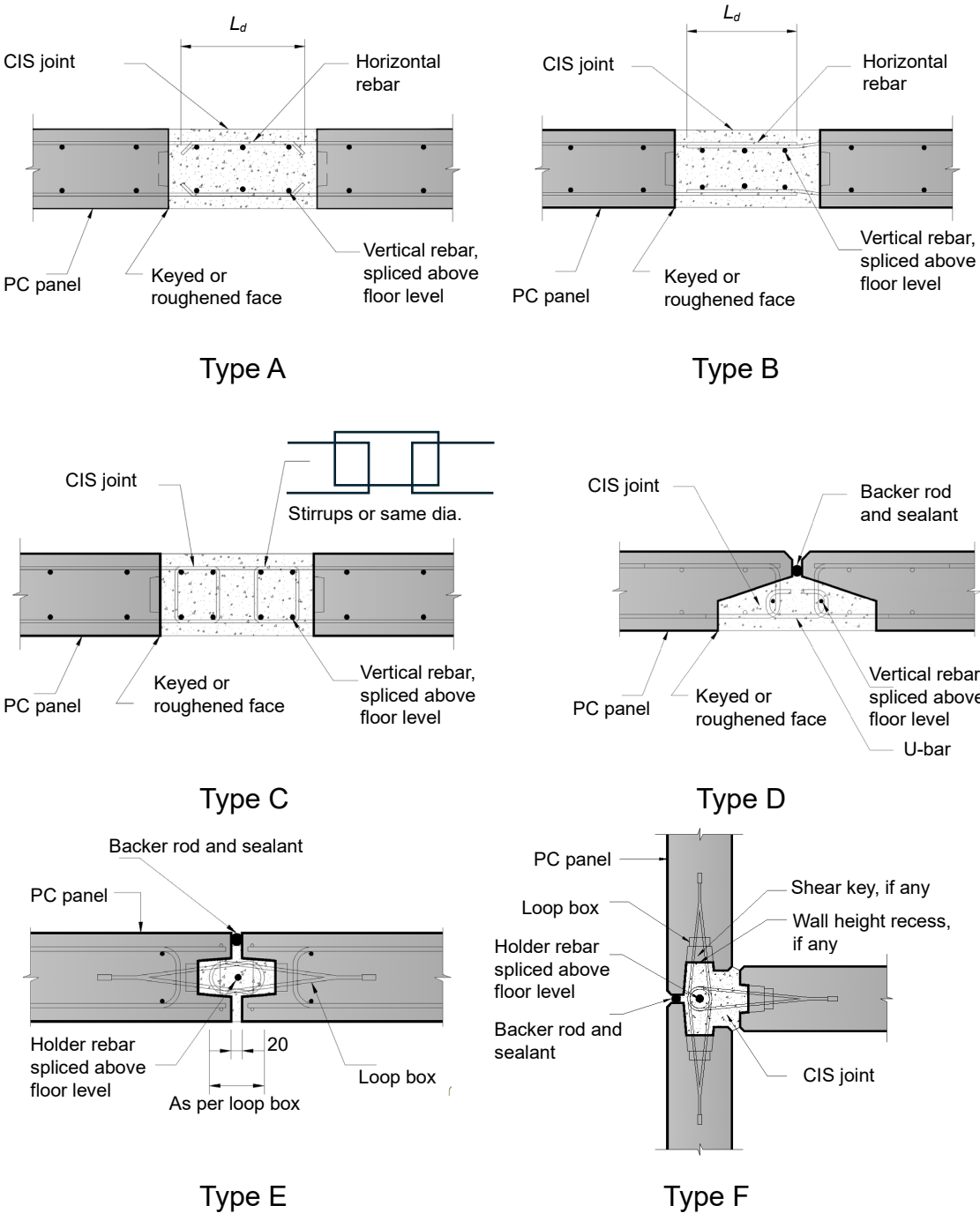
FIG. 56 VERTICAL JOINT BETWEEN WALL TO WALL OR WALL TO COLUMN (Contd.)
