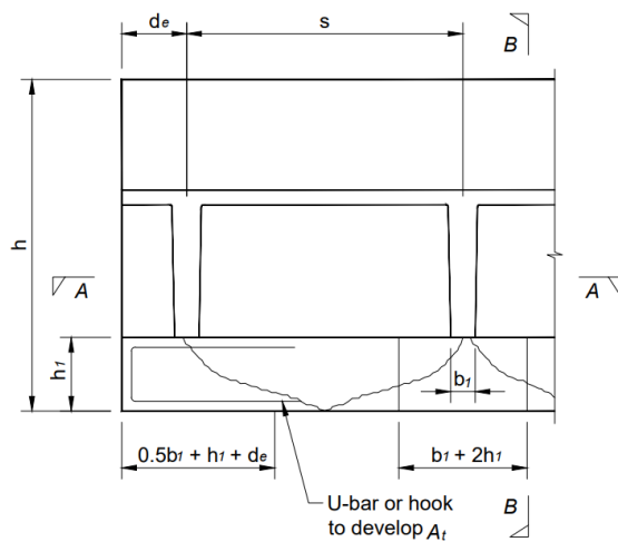
Elavation
