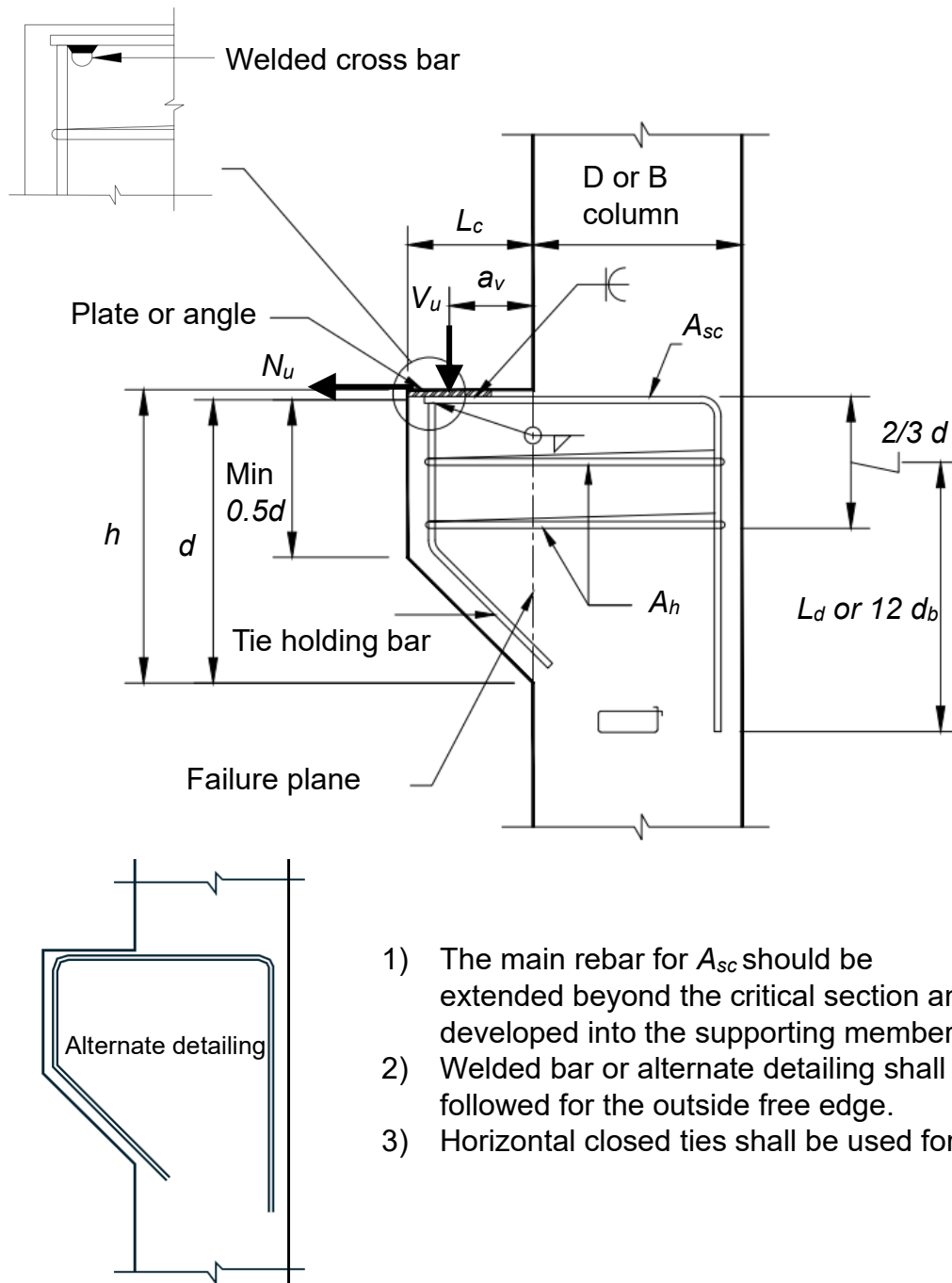
FIG. 28 DESIGN OF CONCRETE CORBELS
