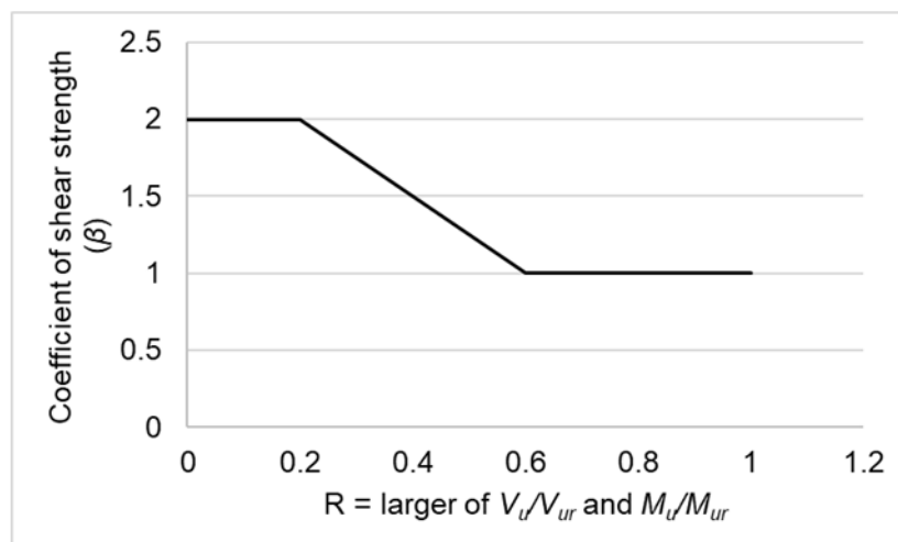
FIG. 26 COEFFICIENT OF SHEAR STRENGTH ( \beta )
