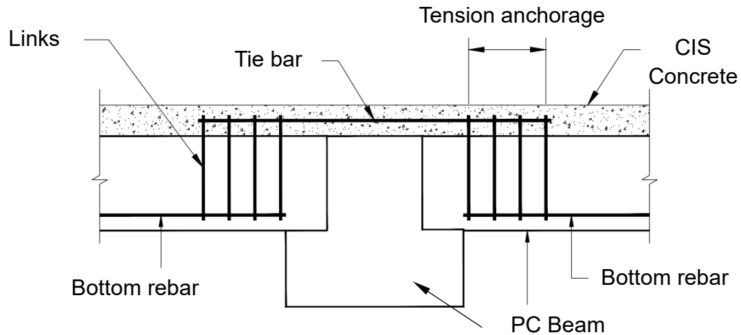
FIG. 37 CONTINUITY OF TIES: ANCHORAGE BY ENCLOSING LINKS
