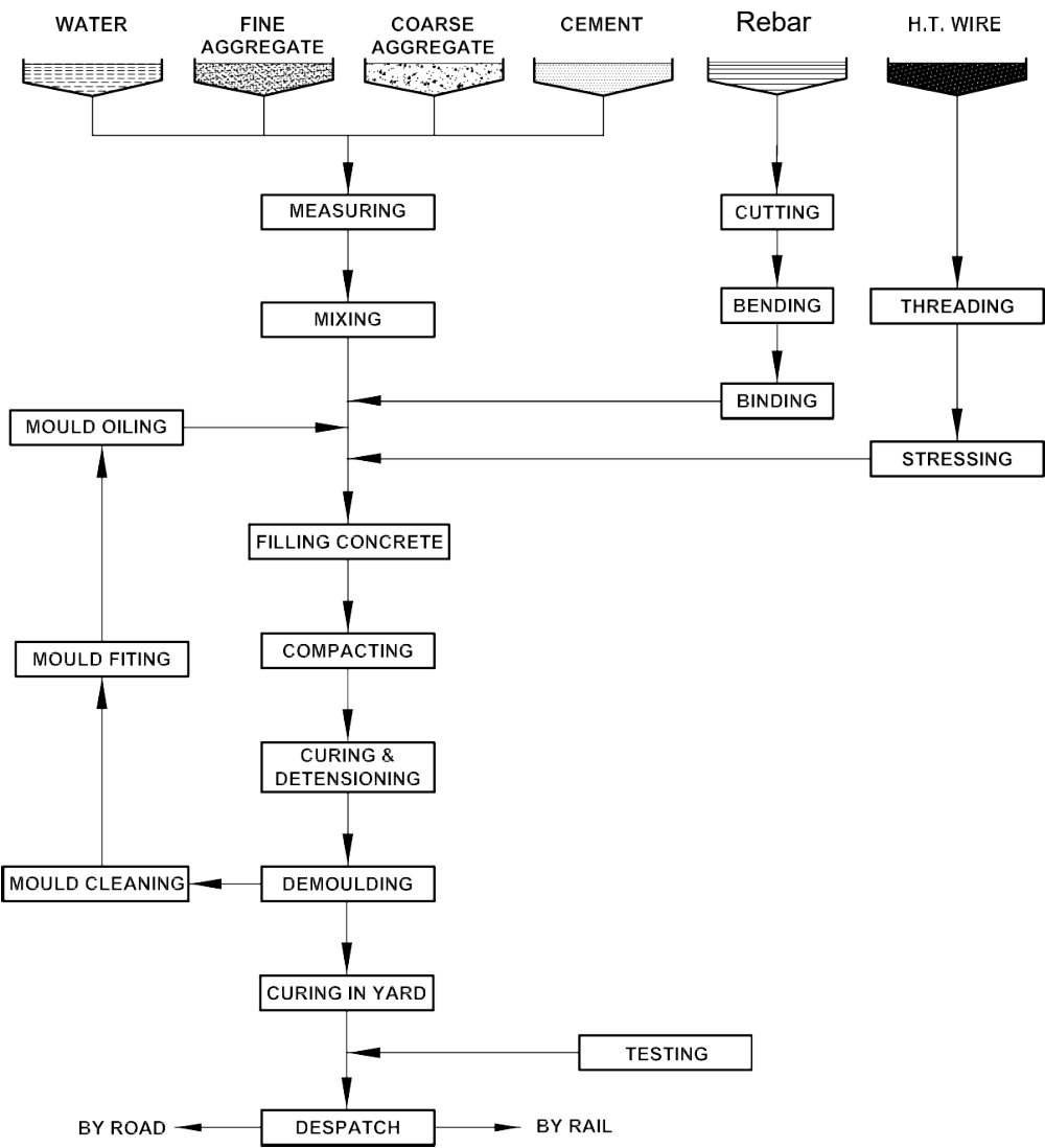
FIG. 40 PLANT PROCESS
