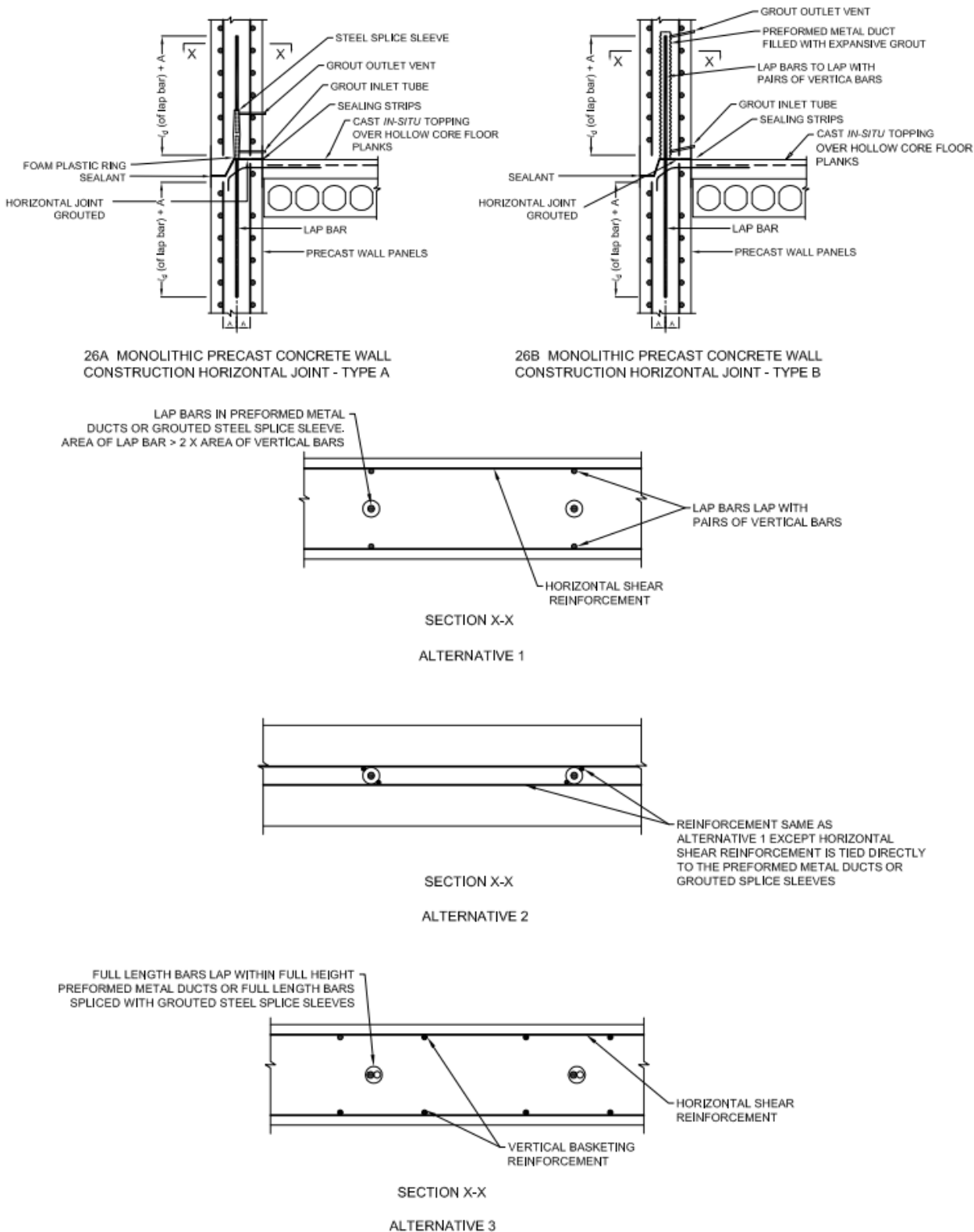
FIG. 55 MONOLITHIC PRECAST WALL CONSTRUCTION
