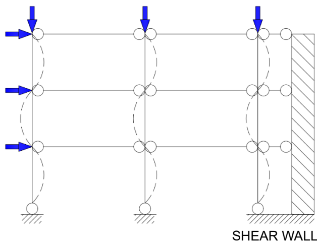
FIG. 5 BRACED FRAMES
