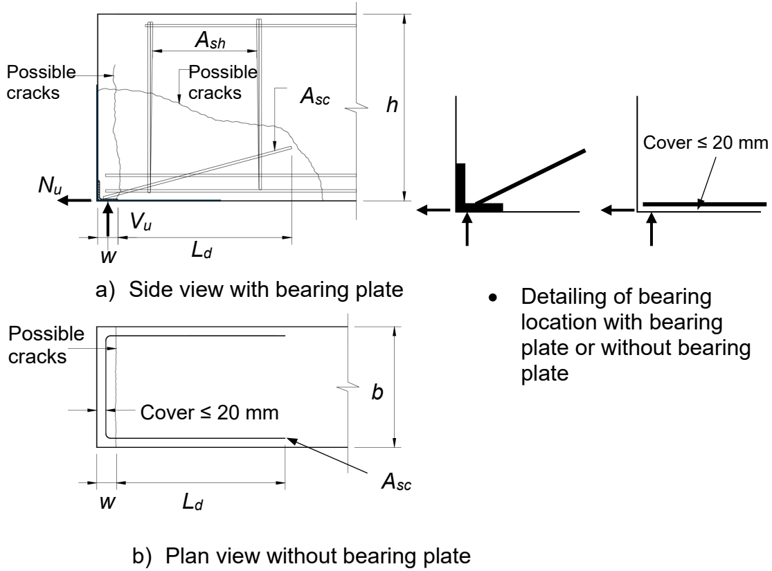
FIG. 21 REINFORCED CONCRETE BEARING
