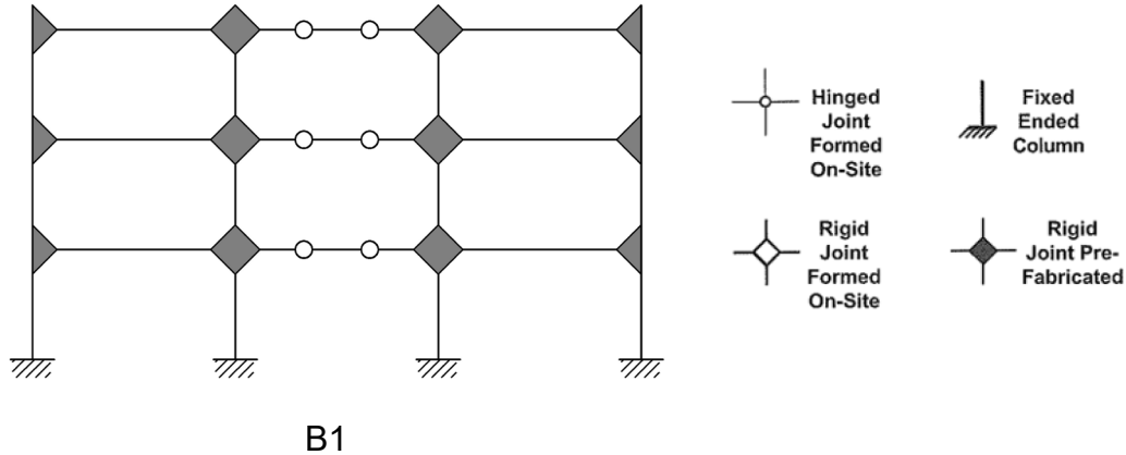
FIG. 3 TYPE B FRAME
