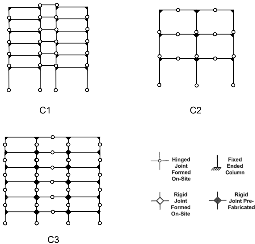
FIG. 4 TYPE C SYSTEMS
