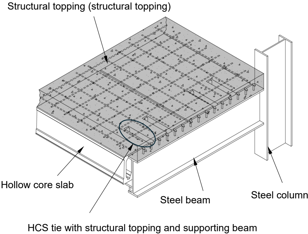
FIG. 11 MIXED SYSTEM
