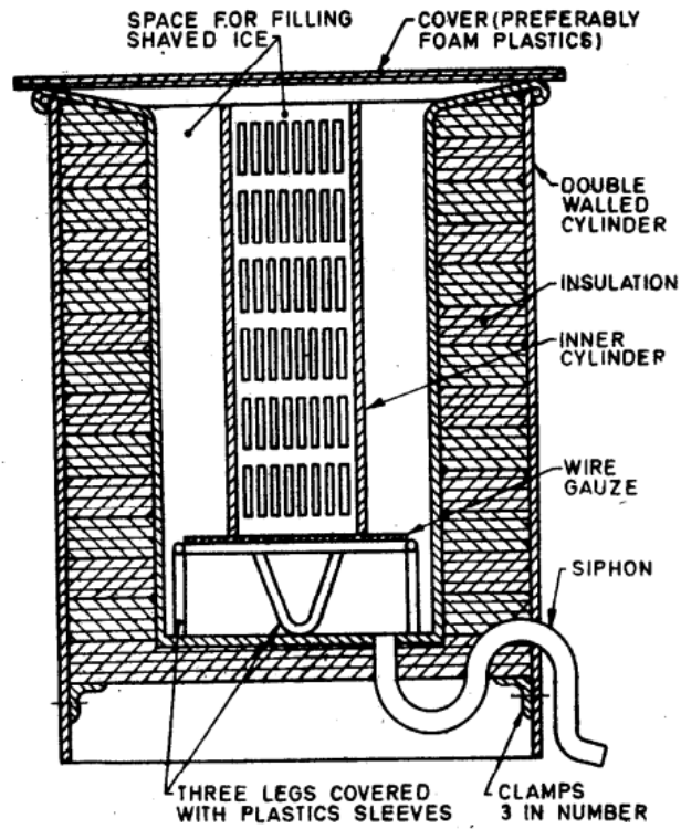
FIG. 1 ICE-POINT EQUIPMENT
