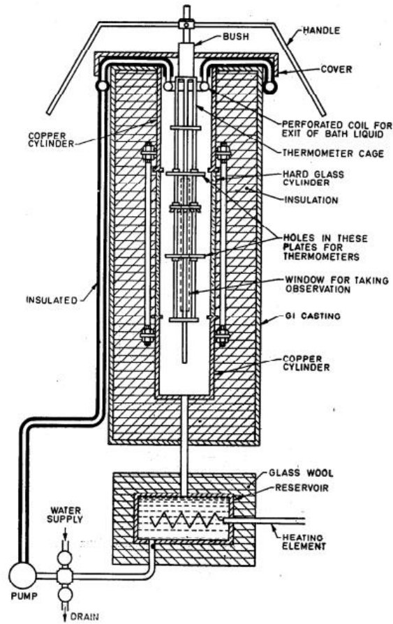
FIG. 4 COMPARATOR BATH, PUMP TYPE
