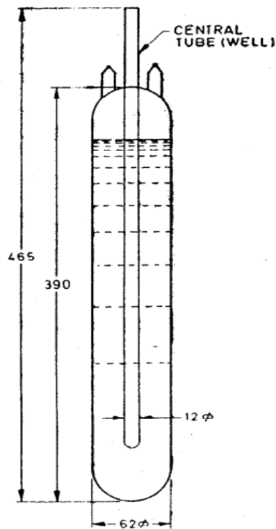
FIG. 2 TRIPLE-POINT-OF-WATER-CELL
