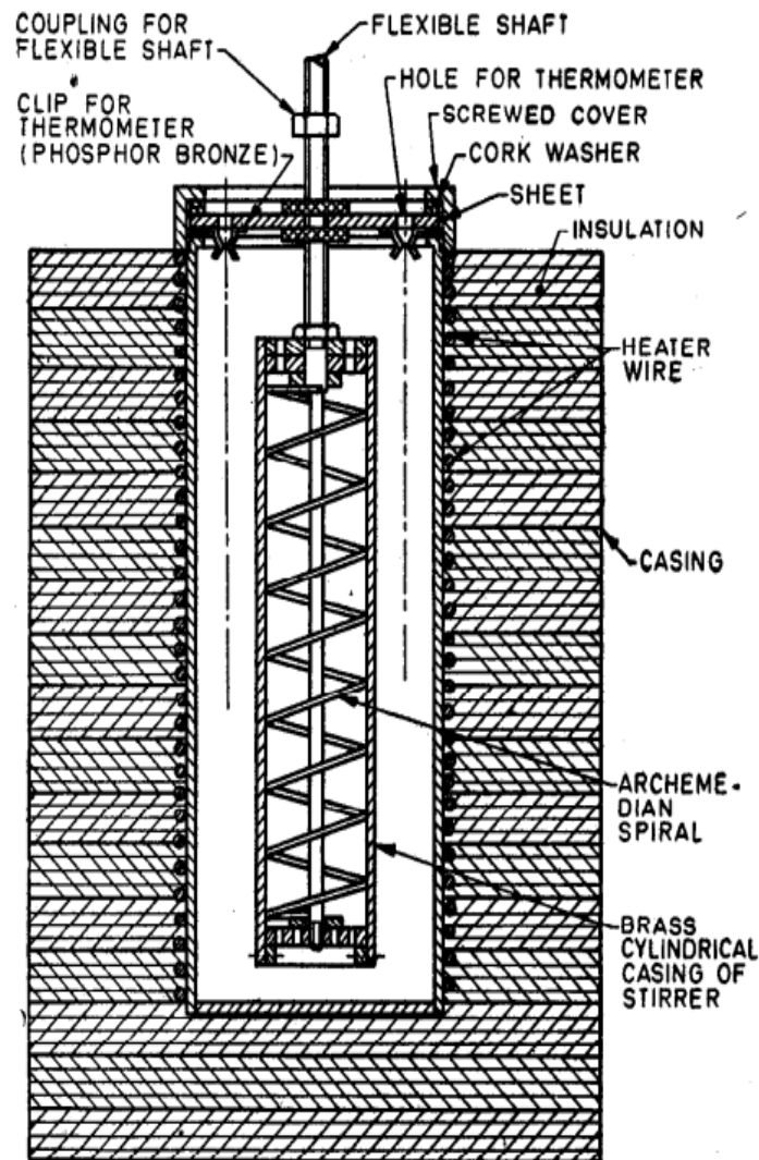
FIG. 3 COMPARATOR BATH, SCREW TYPE
