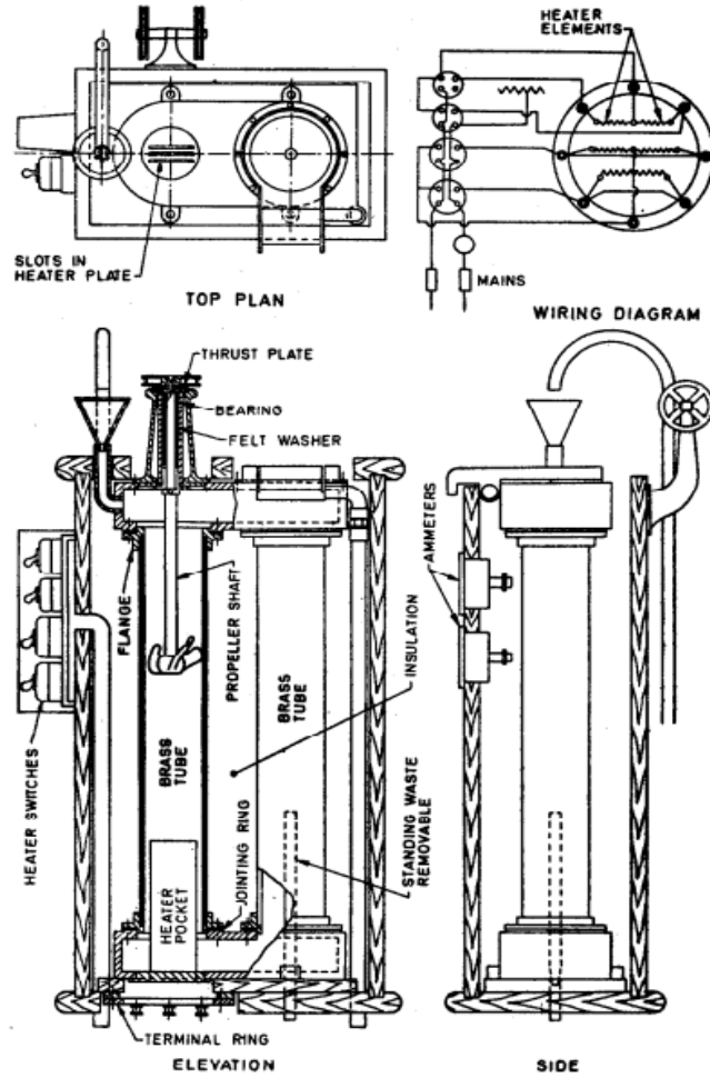
FIG. 6 COMPARATOR BATH, PROPELLER TYPE
