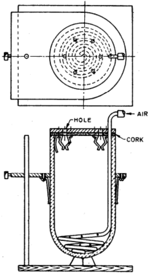
FIG. 5 COMPARATOR BATH, BUBBLER TYPE
