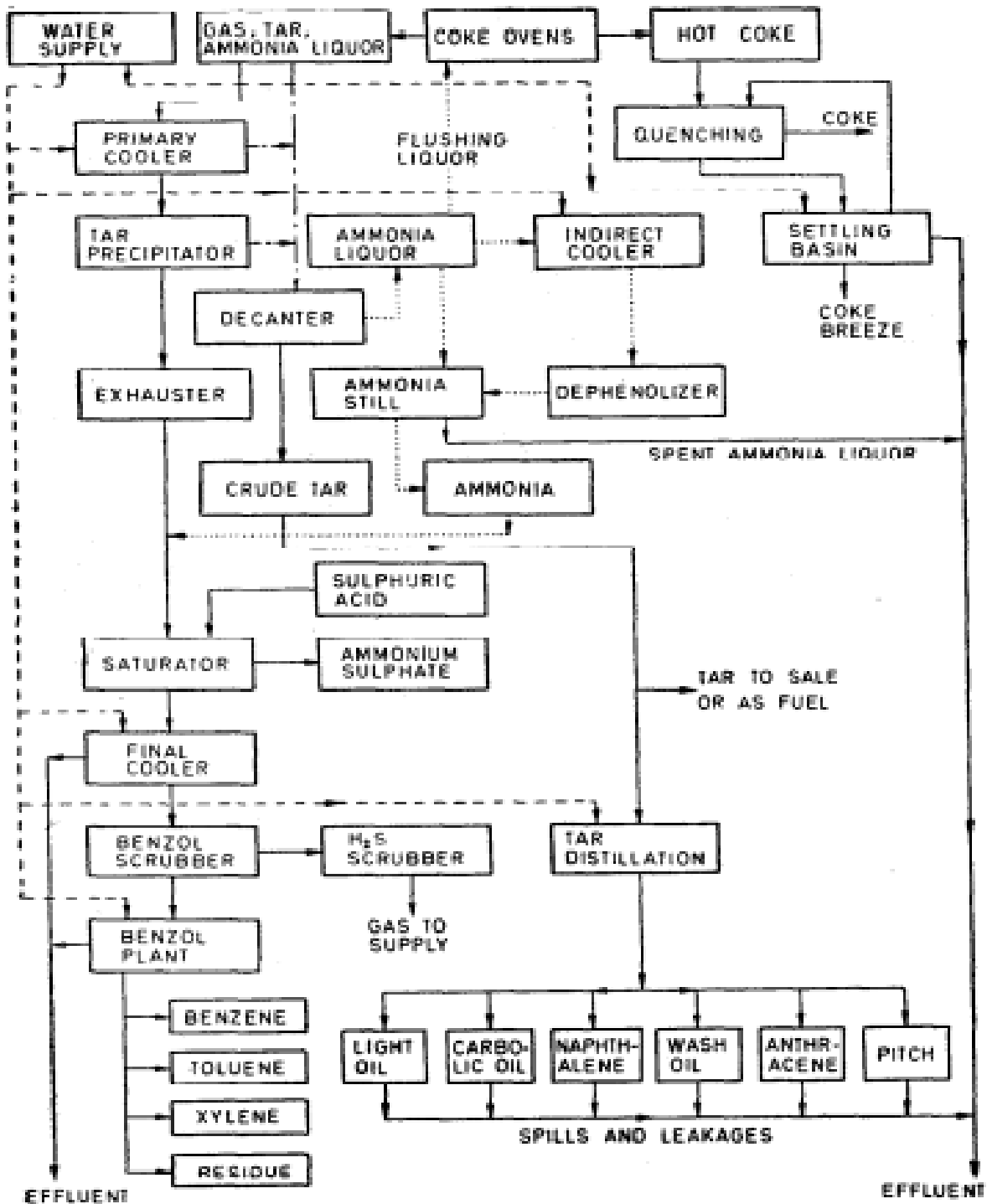
FIG.1 FLOW SHEET OF COKE OVEN BY-PRODUCT PLANT
