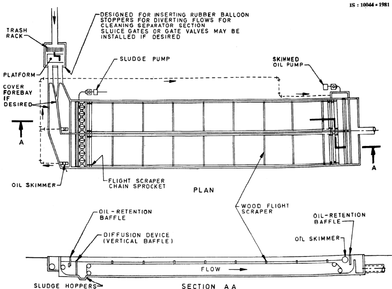
FIG. 1 API OIL-WATER SEPARATOR
