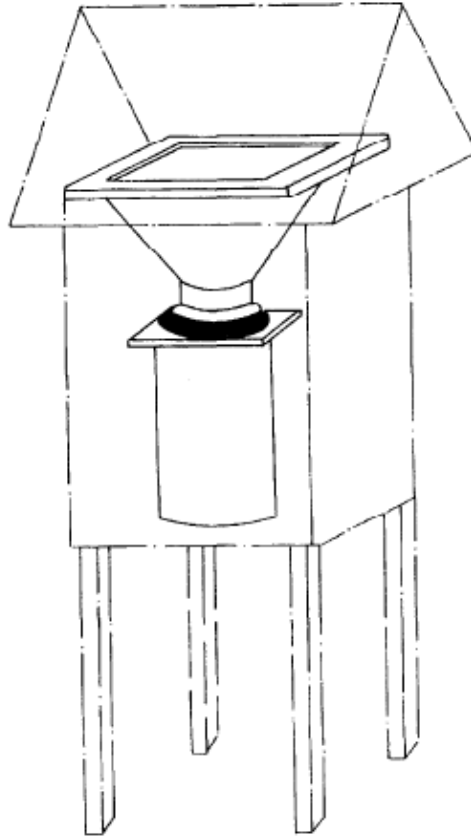
FIG. 1 SAMPLER AND SHELTER
