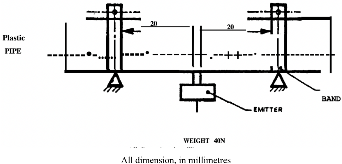
FIG. 1 ON-LINE EMITTER PULL-OUT TEST
