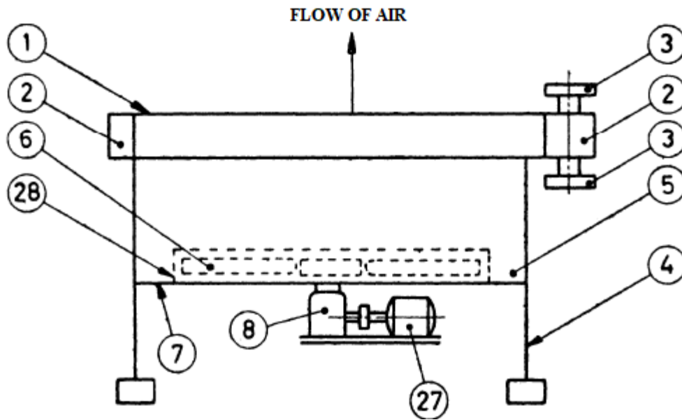
FIG. 2 FORCED DRAFT
