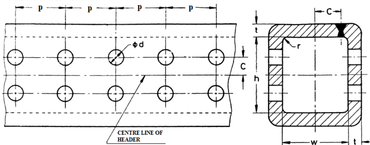
FIG. 9 RECTANGULAR HEADER DESIGN VIEW
