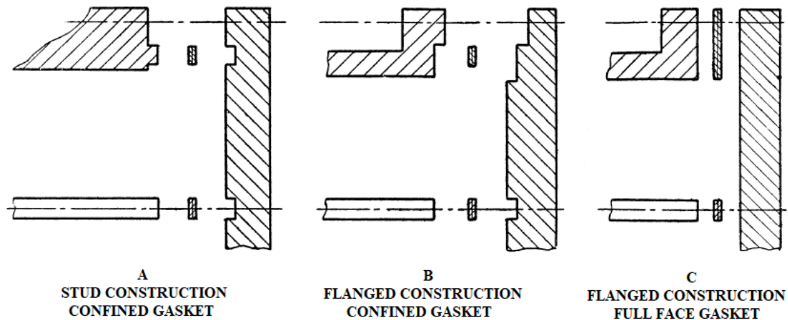
FIG. 7 TYPICAL CONFINED AND FULL-FACE GASKET JOINT DETAILS
