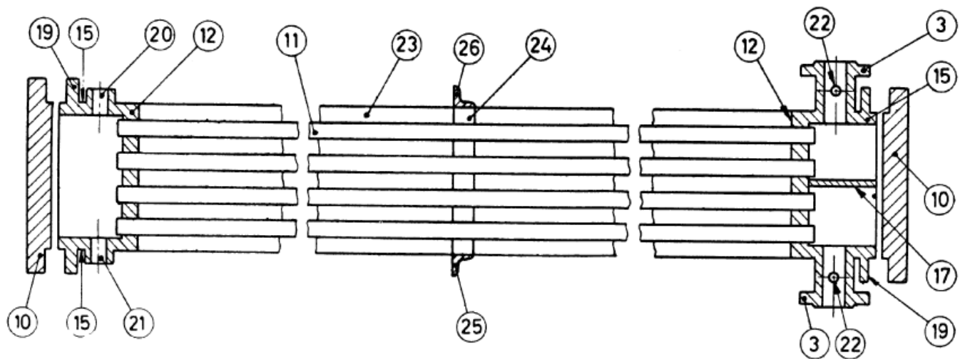
FIG. 5 TYPICAL CONSTRUCTION OF A TUBE BUNDLE WITH REMOVABLE-COVER-PLATE HEADERS
