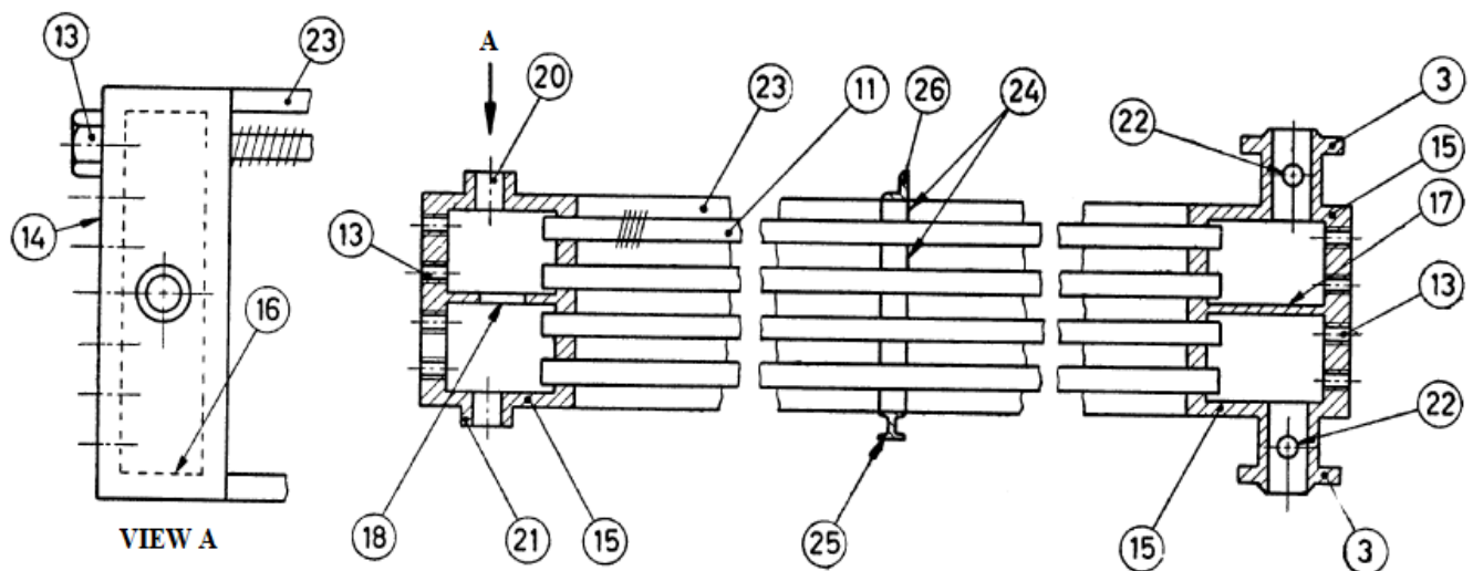
FIG. 6 TYPICAL CONSTRUCTION OF A TUBE BUNDLE WITH PLUG HEADERS
