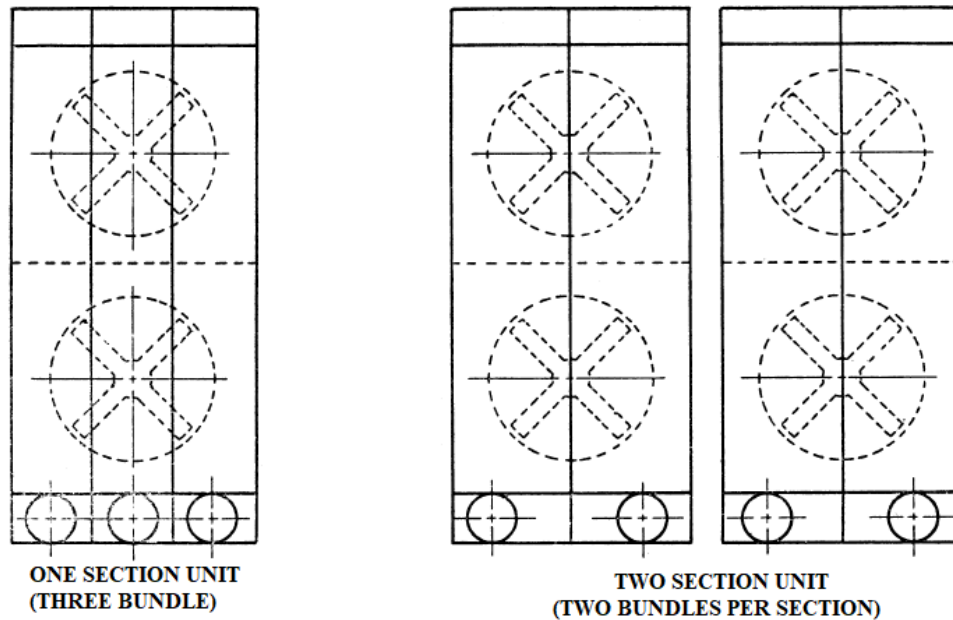
FIG. 1 TYPICAL SECTIONAL ARRANGEMENTS
