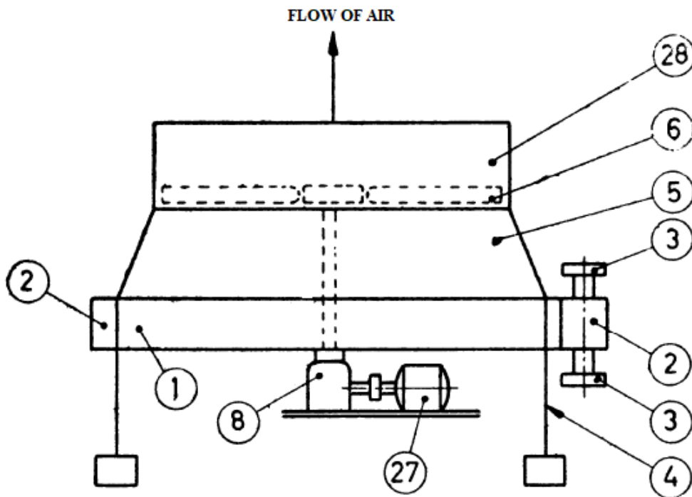
FIG. 3 INDUCED DRAFT
