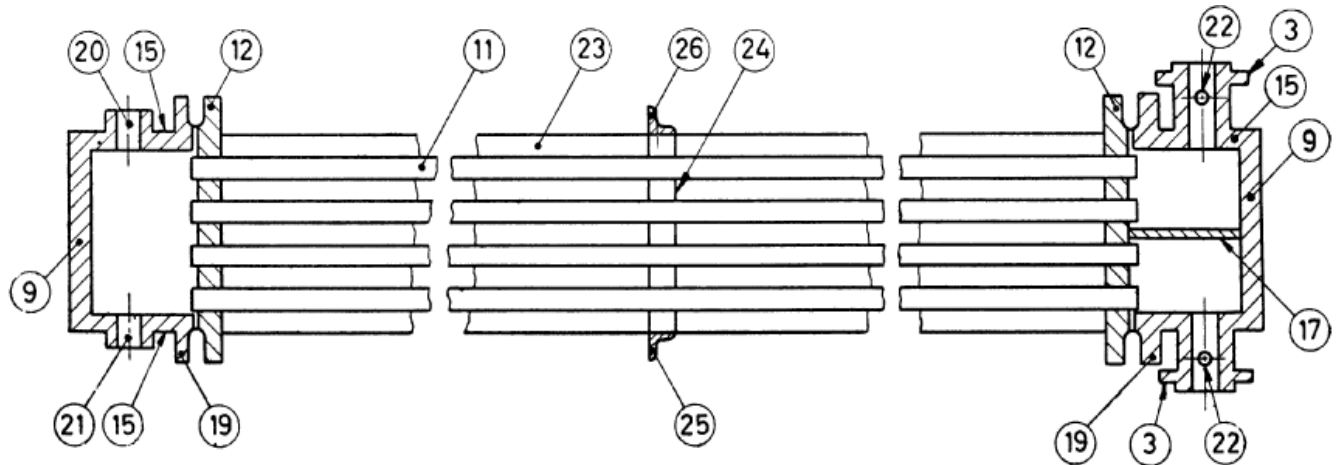
FIG. 4 TYPICAL CONSTRUCTION OF A TUBE BUNDLE WITH REMOVABLE-BONNET HEADERS
