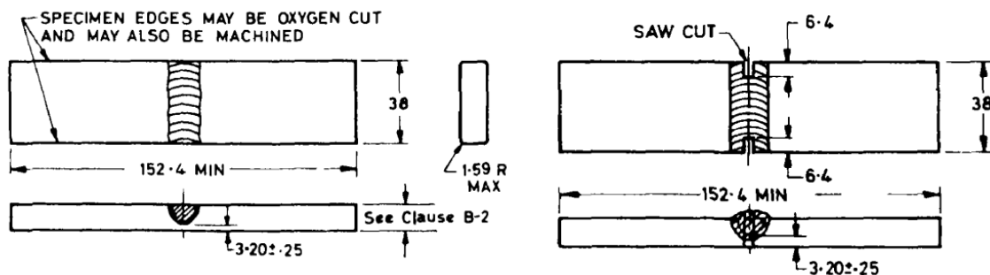
FIG. 4 TENSILE ELONGATION TEST SPECIMEN
