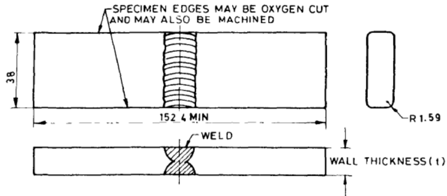
FIG. 3 TRANSVERSE TENSILE TEST SPECIMEN
