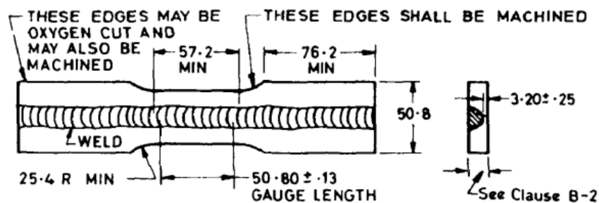
FIG. 4 TENSILE ELONGATION TEST SPECIMEN
