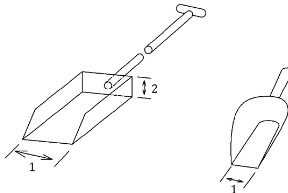
FIG. 3 EXAMPLES OF SCOOPS
