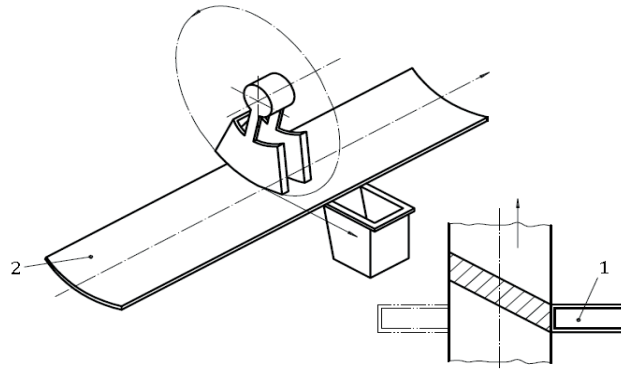
FIG. 13 EXAMPLE OF A CROSS-BELT SAMPLER
