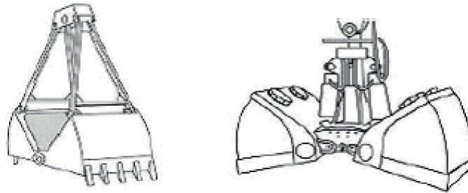
FIG. 6 EXAMPLES OF GRABS (OPEN AND CLOSED TYPE)
