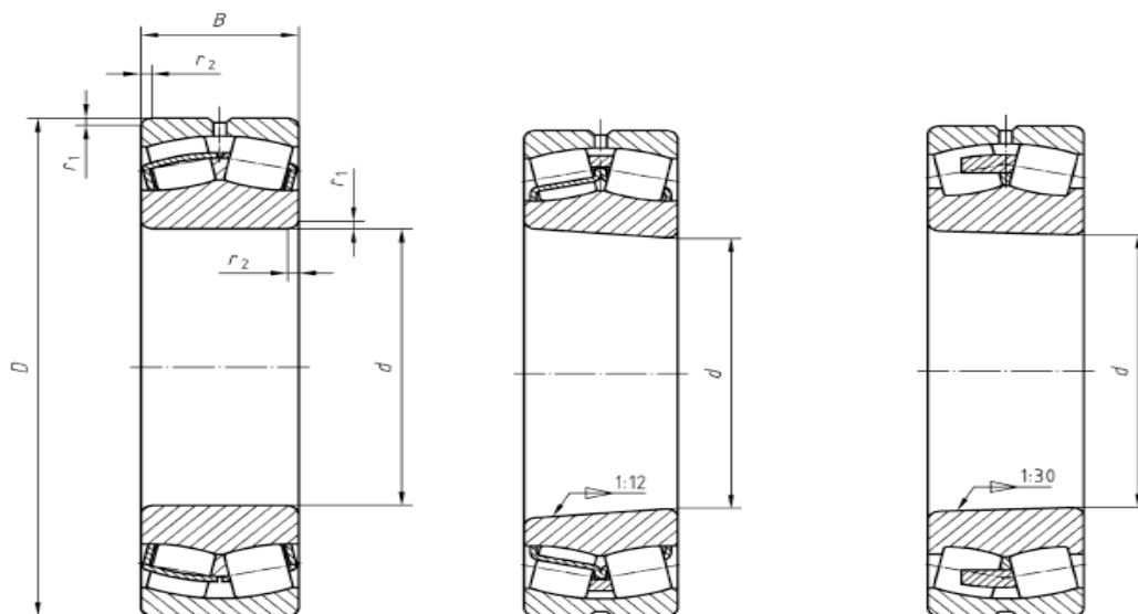
a) Bearing with cylindrical bore b) Bearing with 1:12 tapered bore c) Bearing with 1:30 tapered bore
