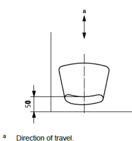
FIG. 1 FRONT-SEATED OPERATOR
