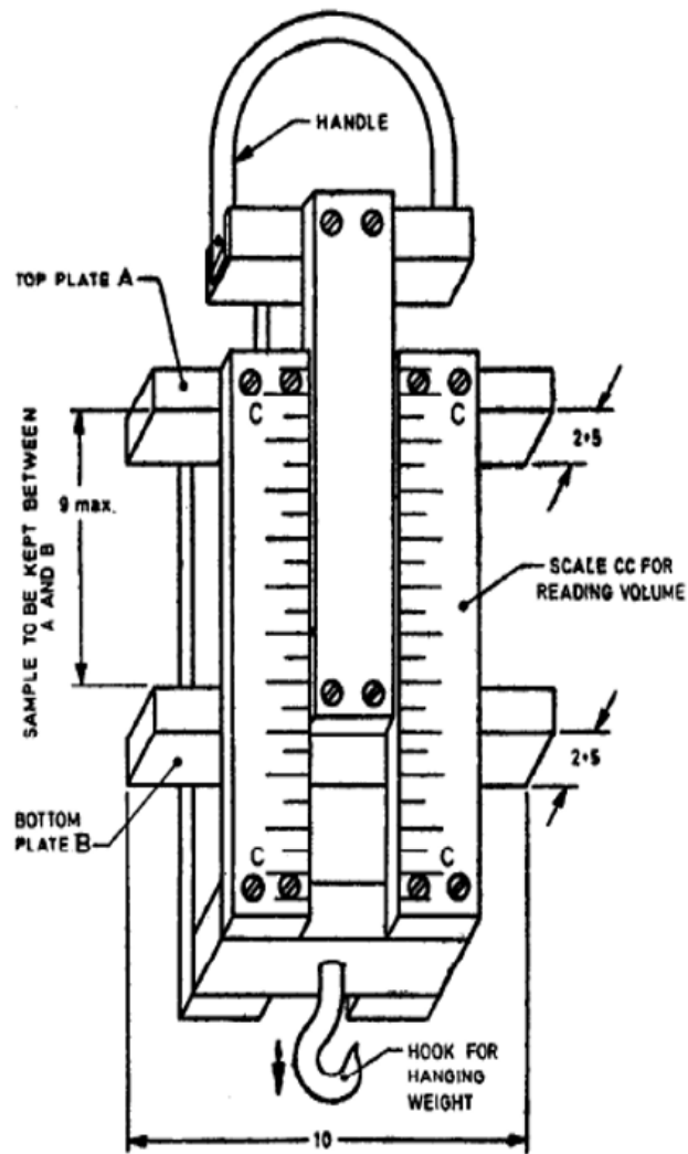
FIG. 1 BULK DENSITY MEASURING GADGET
