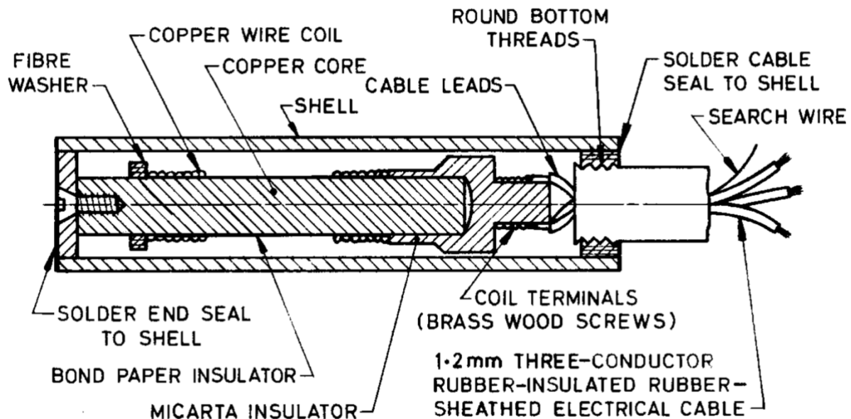
FIG. 1 EMBEDDED TYPE RESISTANCE THERMOMETER
