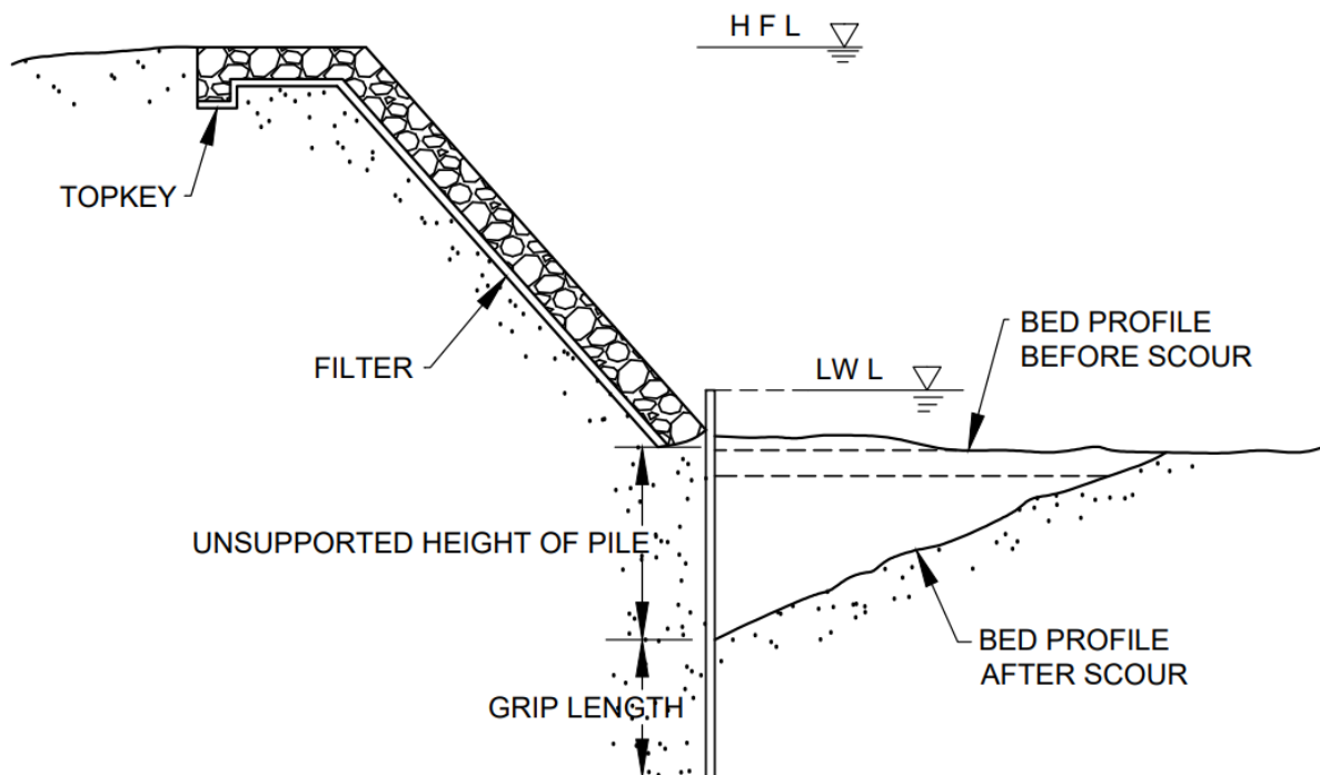
FIG. 6 TOE PROTECTION WITH PILE AND TOE KEY
