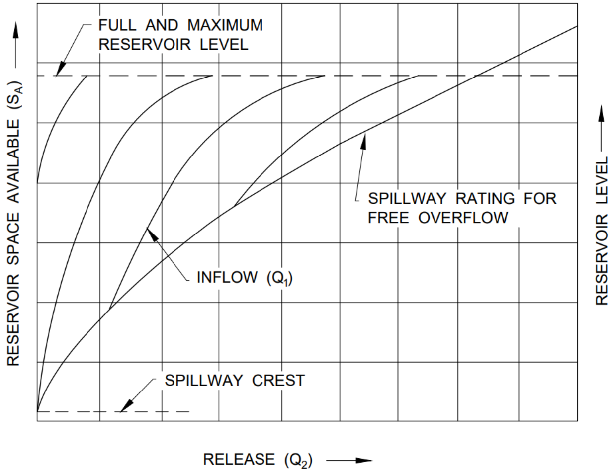
FIG. 2 SPILLWAY GATE REGULATION SCHEDULE WITHOUT INDUCED SURCHARGE
